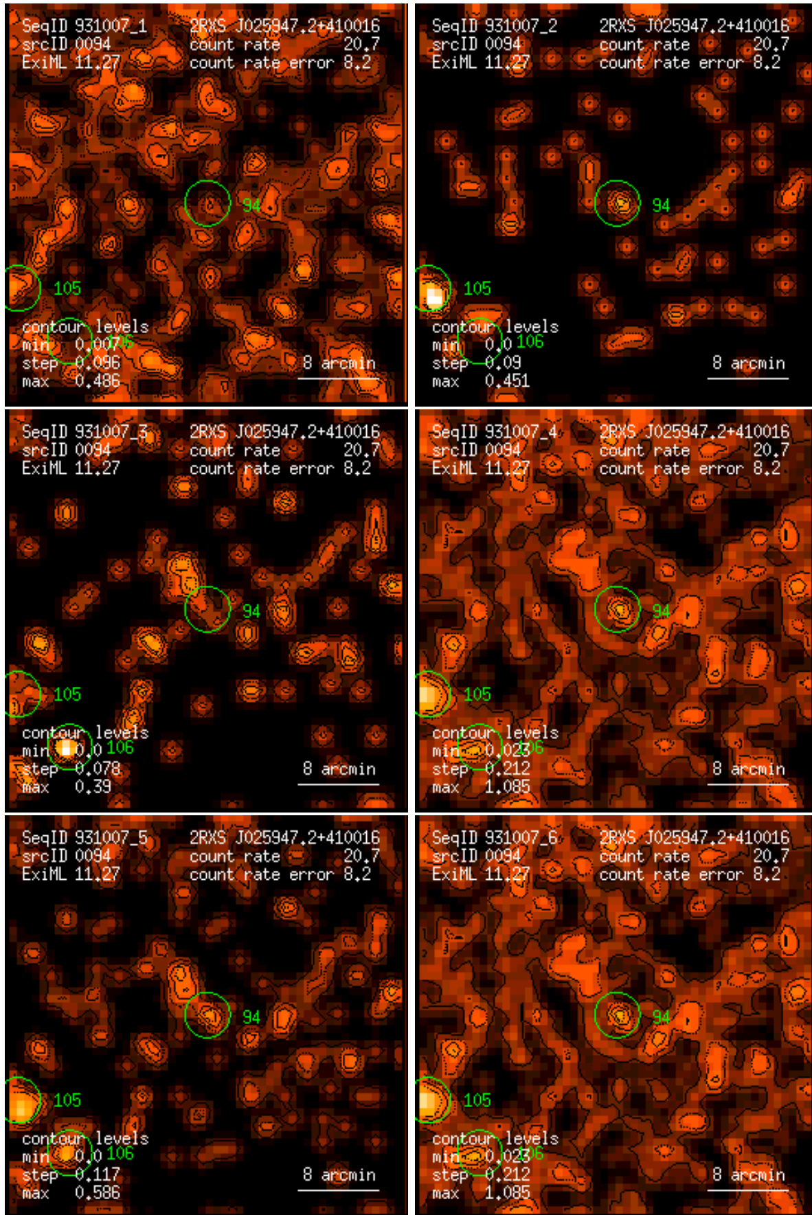
Figure 94: RASS 931007: detection 0094: band rate images, Gaussian filter: (1) PSPC channels 11 – 41, (2) 52 – 90, (3) 91 – 201, (4) 11 – 235, (5) 52 – 201, (6) 11 – 201. Broad band rates in counts/ks. Band rate contour levels in counts/ks/arcmin 2 .
