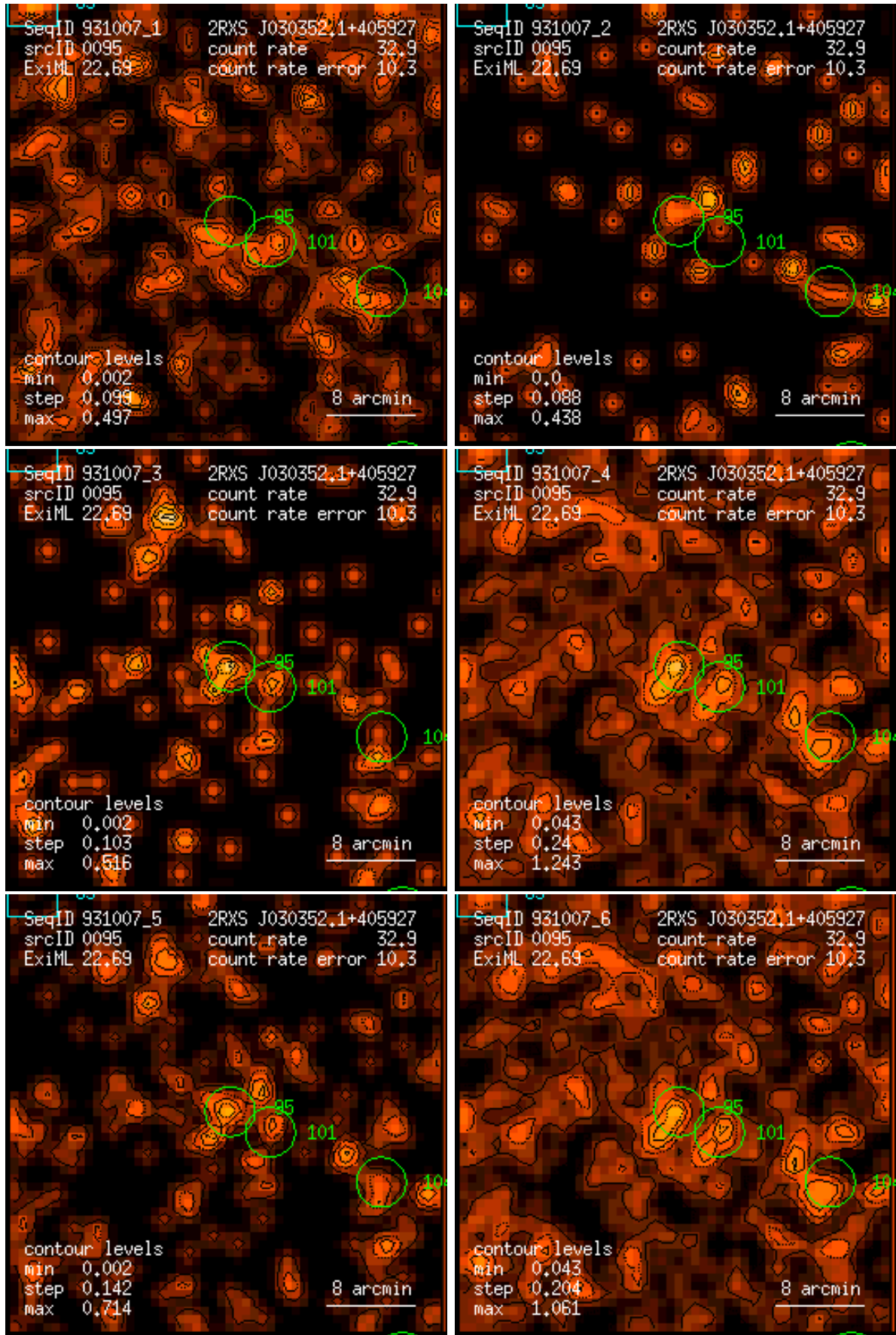
Figure 95: RASS 931007: detection 0095: band rate images, Gaussian filter: (1) PSPC channels 11 – 41, (2) 52 – 90, (3) 91 – 201, (4) 11 – 235, (5) 52 – 201, (6) 11 – 201. Broad band rates in counts/ks. Band rate contour levels in counts/ks/arcmin 2 .
