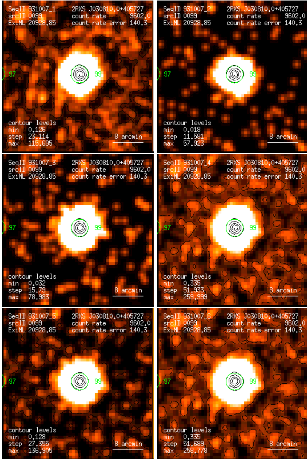
Figure 99: RASS 931007: detection 0099: band rate images, Gaussian filter: (1) PSPC channels 11 – 41, (2) 52 – 90, (3) 91 – 201, (4) 11 – 235, (5) 52 – 201, (6) 11 – 201. Broad band rates in counts/ks. Band rate contour levels in counts/ks/arcmin 2 .
