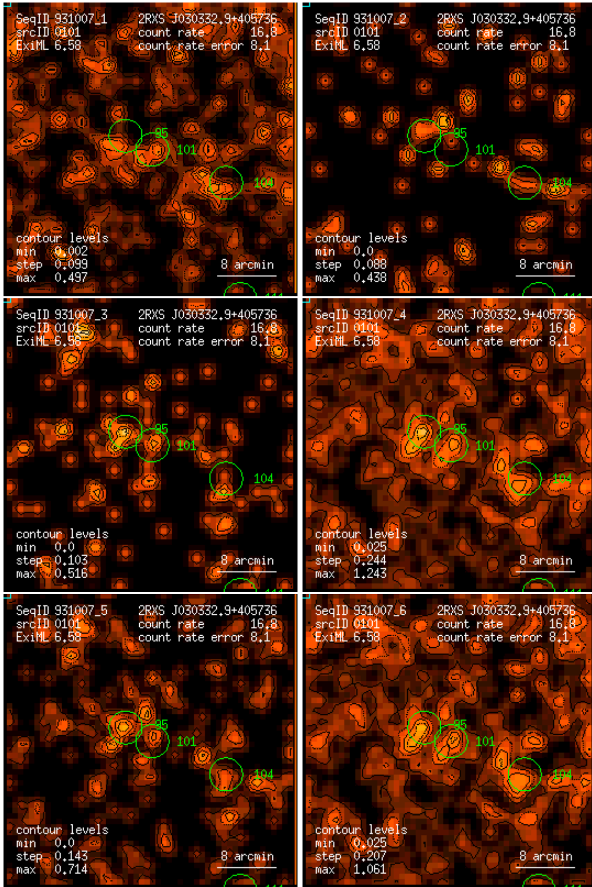
Figure 101: RASS 931007: detection 0101: band rate images, Gaussian filter: (1) PSPC channels 11 – 41, (2) 52 – 90, (3) 91 – 201, (4) 11 – 235, (5) 52 – 201, (6) 11 – 201. Broad band rates in counts/ks. Band rate contour levels in counts/ks/arcmin 2 .
