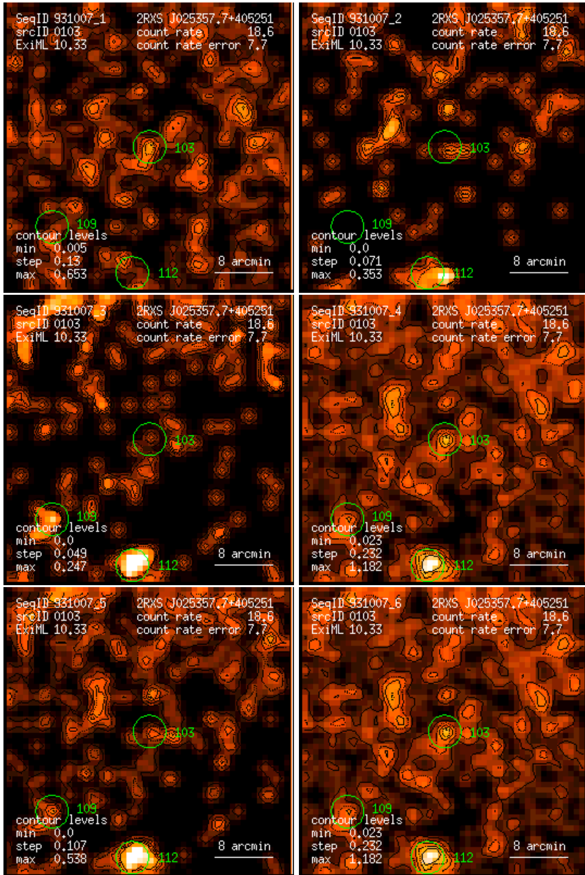
Figure 103: RASS 931007: detection 0103: band rate images, Gaussian filter: (1) PSPC channels 11 – 41, (2) 52 – 90, (3) 91 – 201, (4) 11 – 235, (5) 52 – 201, (6) 11 – 201. Broad band rates in counts/ks. Band rate contour levels in counts/ks/arcmin 2 .
