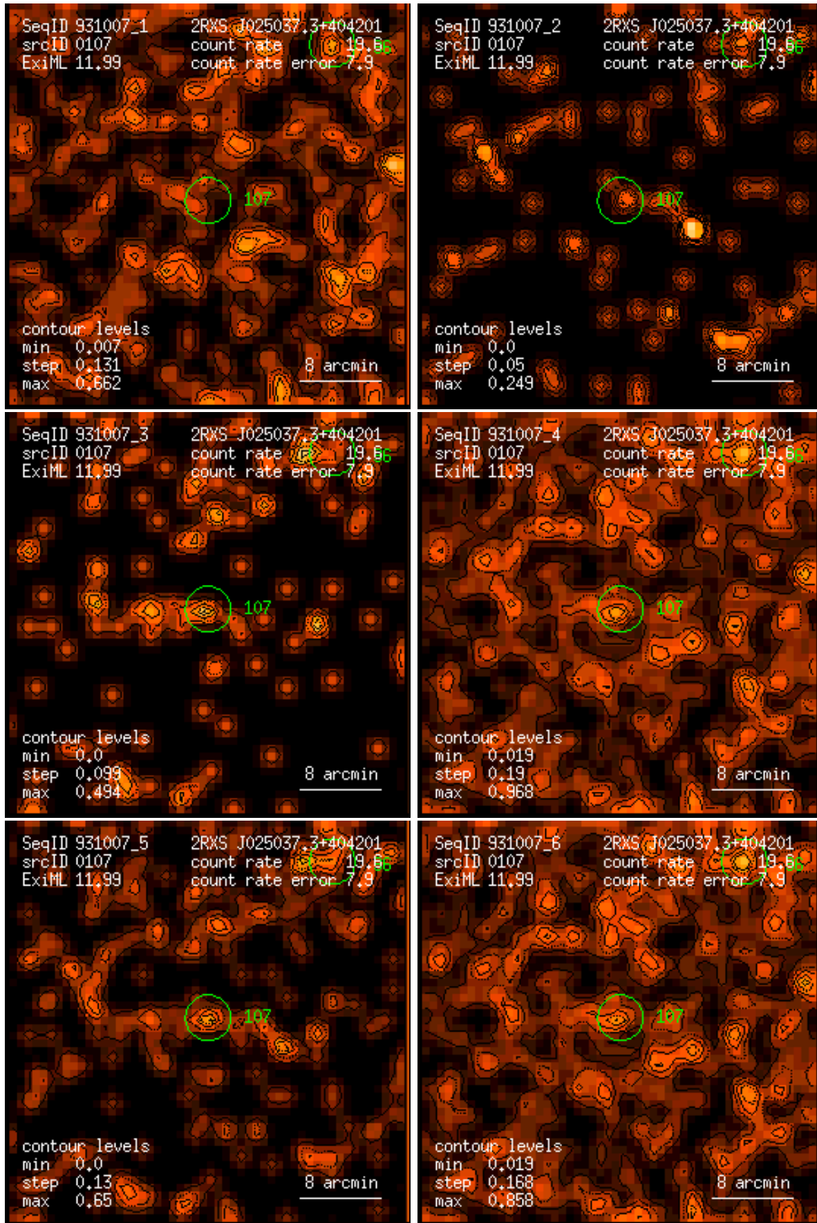
Figure 107: RASS 931007: detection 0107: band rate images, Gaussian filter: (1) PSPC channels 11 – 41, (2) 52 – 90, (3) 91 – 201, (4) 11 – 235, (5) 52 – 201, (6) 11 – 201. Broad band rates in counts/ks. Band rate contour levels in counts/ks/arcmin 2 .
