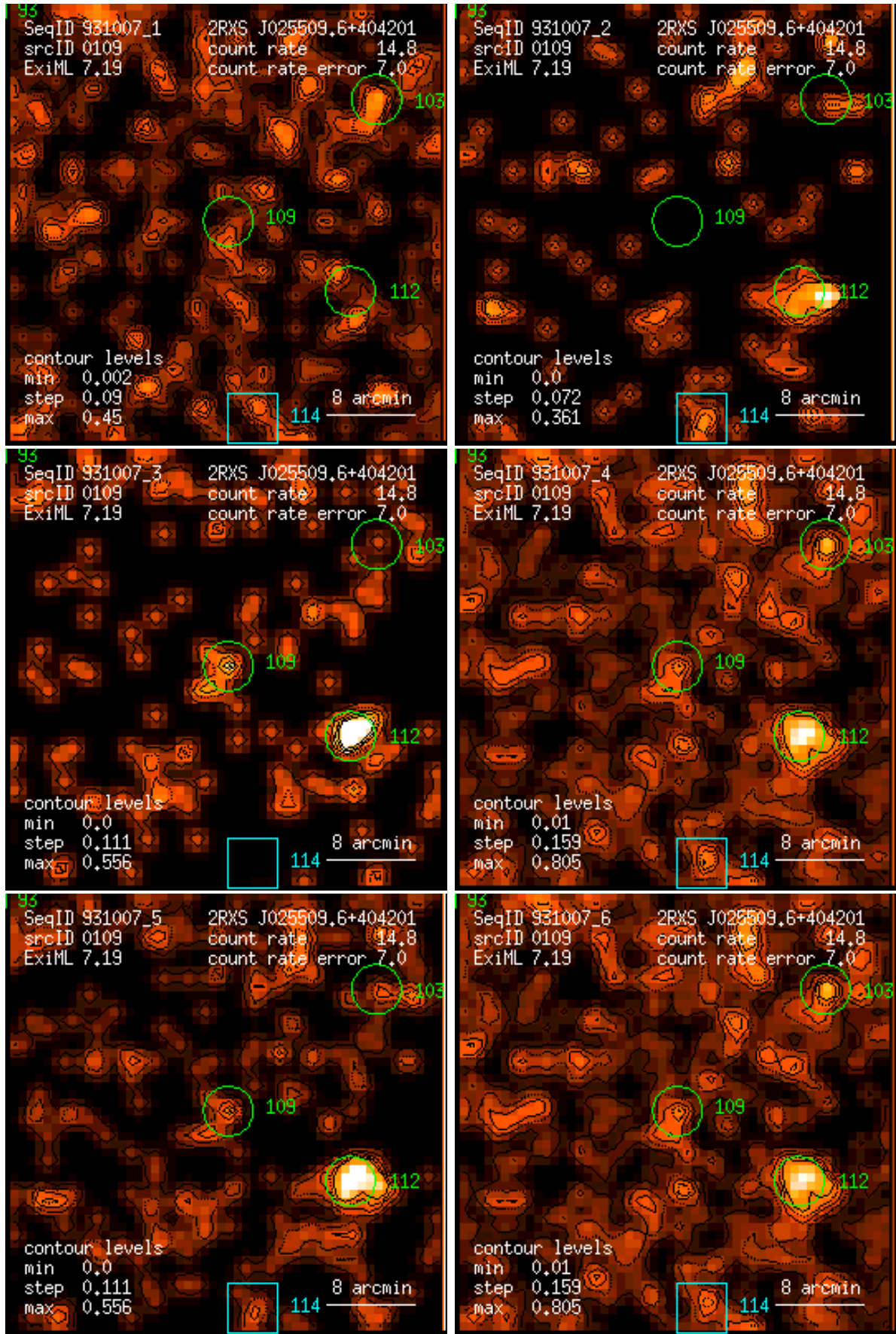
Figure 109: RASS 931007: detection 0109: band rate images, Gaussian filter: (1) PSPC channels 11 – 41, (2) 52 – 90, (3) 91 – 201, (4) 11 – 235, (5) 52 – 201, (6) 11 – 201. Broad band rates in counts/ks. Band rate contour levels in counts/ks/arcmin 2 .
