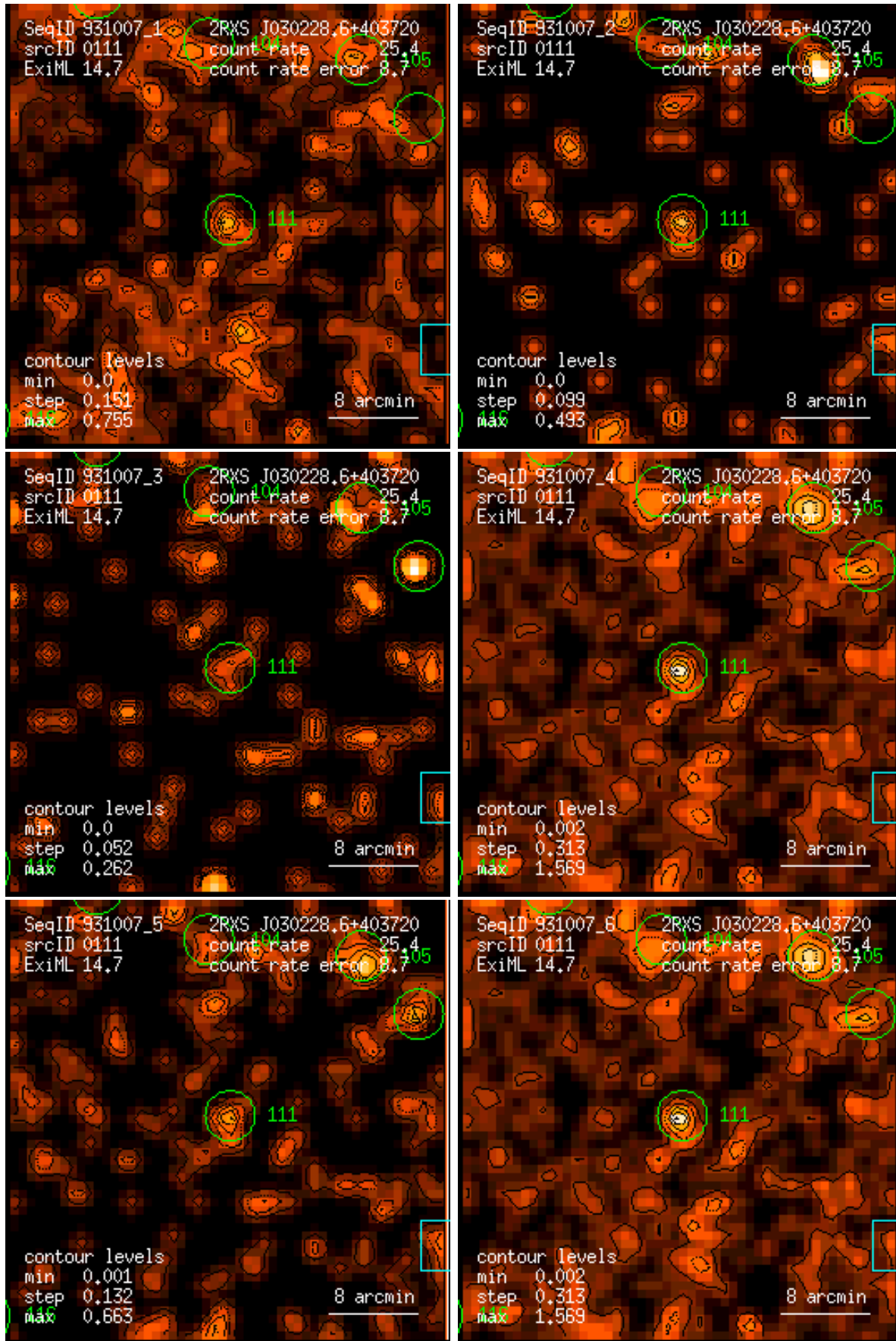
Figure 111: RASS 931007: detection 0111: band rate images, Gaussian filter: (1) PSPC channels 11 – 41, (2) 52 – 90, (3) 91 – 201, (4) 11 – 235, (5) 52 – 201, (6) 11 – 201. Broad band rates in counts/ks. Band rate contour levels in counts/ks/arcmin 2 .
