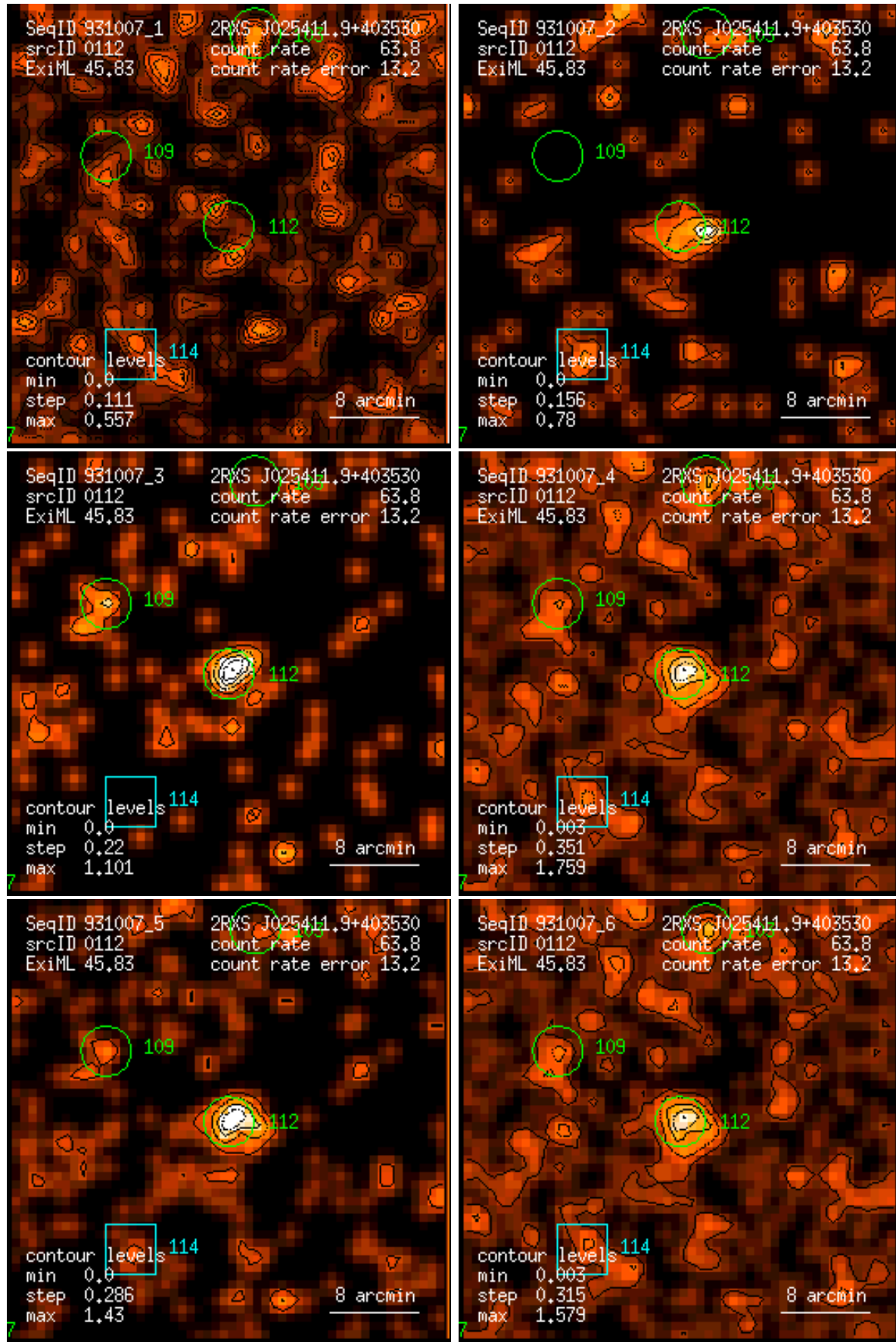
Figure 112: RASS 931007: detection 0112: band rate images, Gaussian filter: (1) PSPC channels 11 – 41, (2) 52 – 90, (3) 91 – 201, (4) 11 – 235, (5) 52 – 201, (6) 11 – 201. Broad band rates in counts/ks. Band rate contour levels in counts/ks/arcmin 2 .
