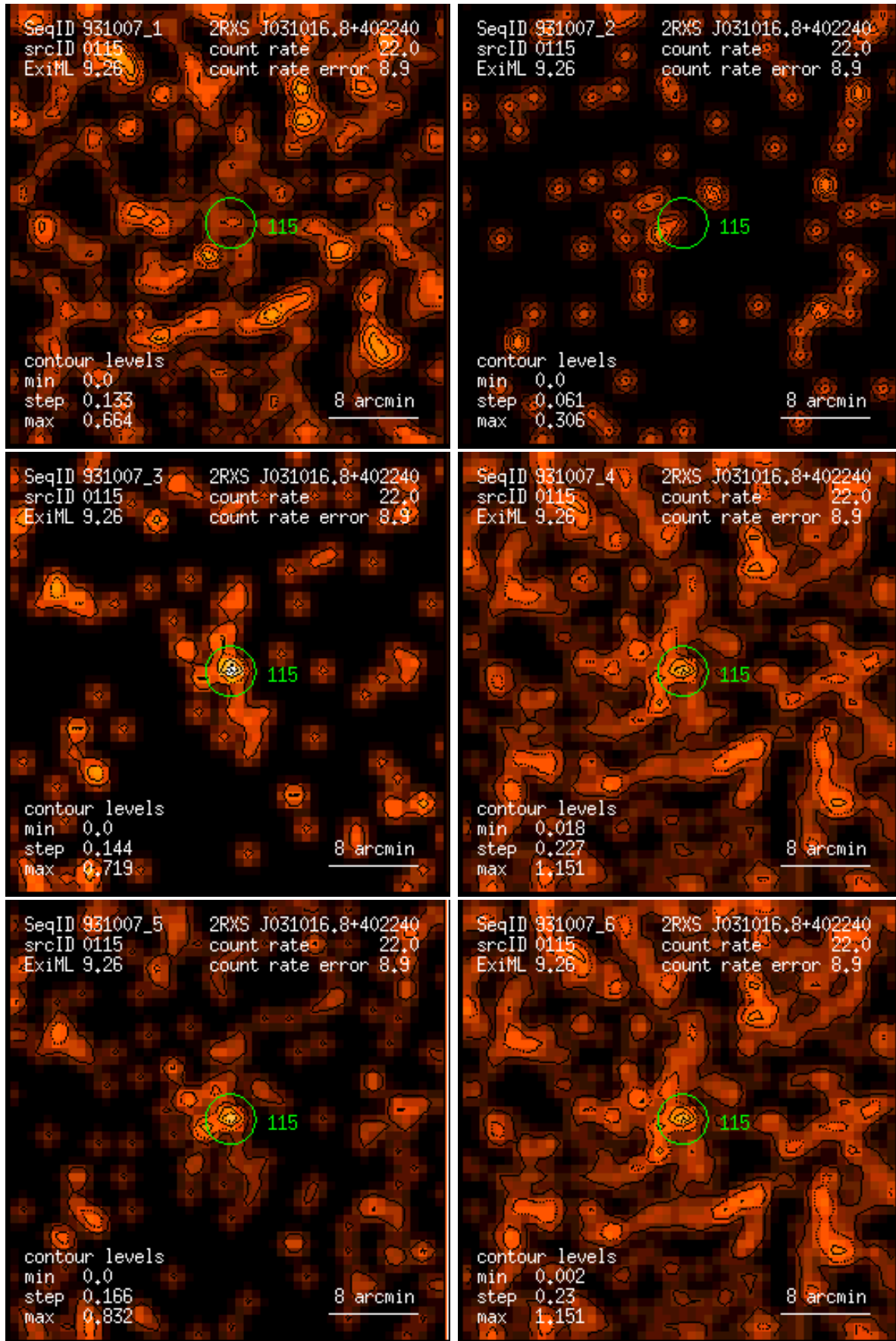
Figure 115: RASS 931007: detection 0115: band rate images, Gaussian filter: (1) PSPC channels 11 – 41, (2) 52 – 90, (3) 91 – 201, (4) 11 – 235, (5) 52 – 201, (6) 11 – 201. Broad band rates in counts/ks. Band rate contour levels in counts/ks/arcmin 2 .
