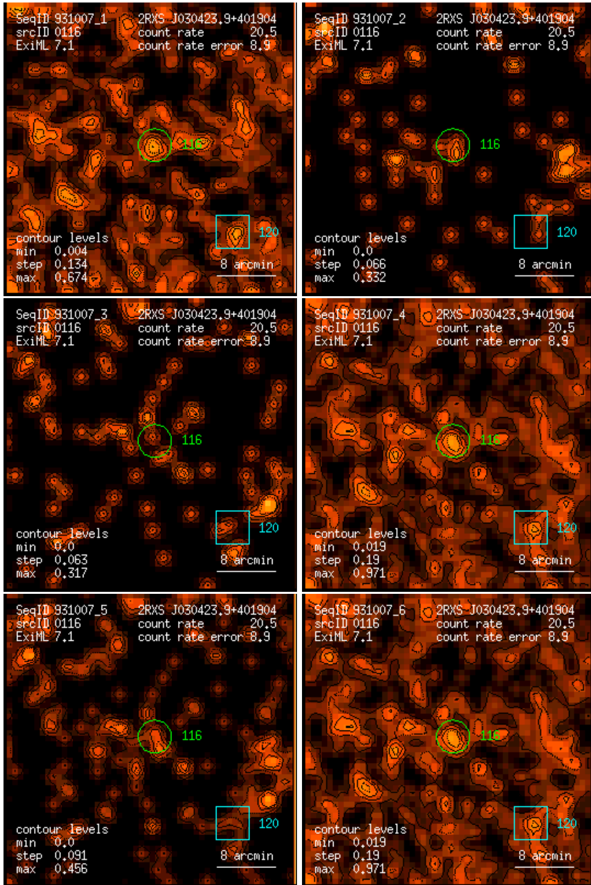
Figure 116: RASS 931007: detection 0116: band rate images, Gaussian filter: (1) PSPC channels 11 – 41, (2) 52 – 90, (3) 91 – 201, (4) 11 – 235, (5) 52 – 201, (6) 11 – 201. Broad band rates in counts/ks. Band rate contour levels in counts/ks/arcmin 2 .
