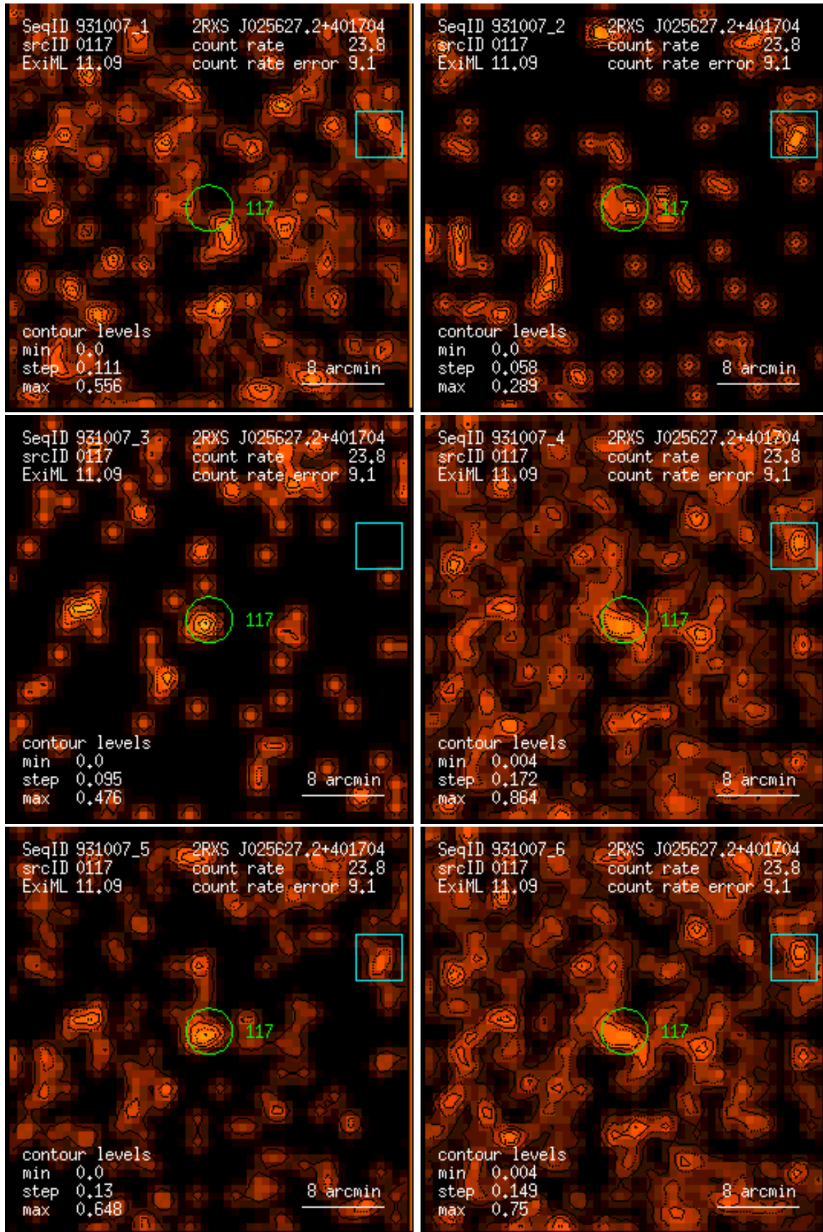
Figure 117: RASS 931007: detection 0117: band rate images, Gaussian filter: (1) PSPC channels 11 – 41, (2) 52 – 90, (3) 91 – 201, (4) 11 – 235, (5) 52 – 201, (6) 11 – 201. Broad band rates in counts/ks. Band rate contour levels in counts/ks/arcmin 2 .
