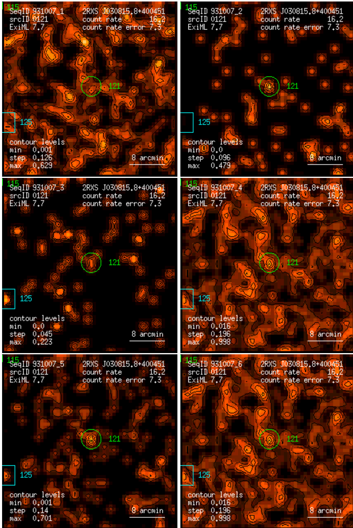
Figure 121: RASS 931007: detection 0121: band rate images, Gaussian filter: (1) PSPC channels 11 – 41, (2) 52 – 90, (3) 91 – 201, (4) 11 – 235, (5) 52 – 201, (6) 11 – 201. Broad band rates in counts/ks. Band rate contour levels in counts/ks/arcmin 2 .
