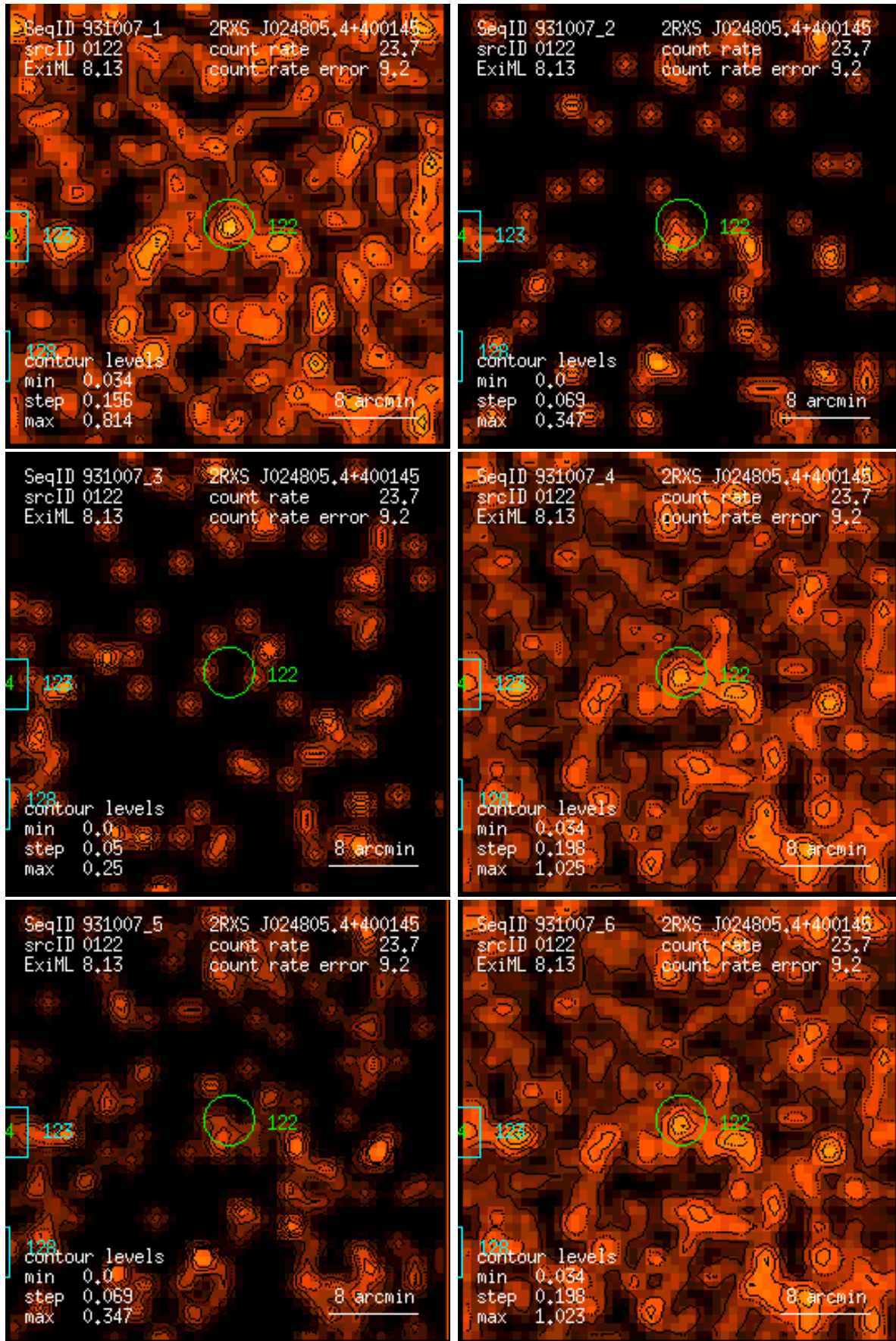
Figure 122: RASS 931007: detection 0122: band rate images, Gaussian filter: (1) PSPC channels 11 – 41, (2) 52 – 90, (3) 91 – 201, (4) 11 – 235, (5) 52 – 201, (6) 11 – 201. Broad band rates in counts/ks. Band rate contour levels in counts/ks/arcmin 2 .
