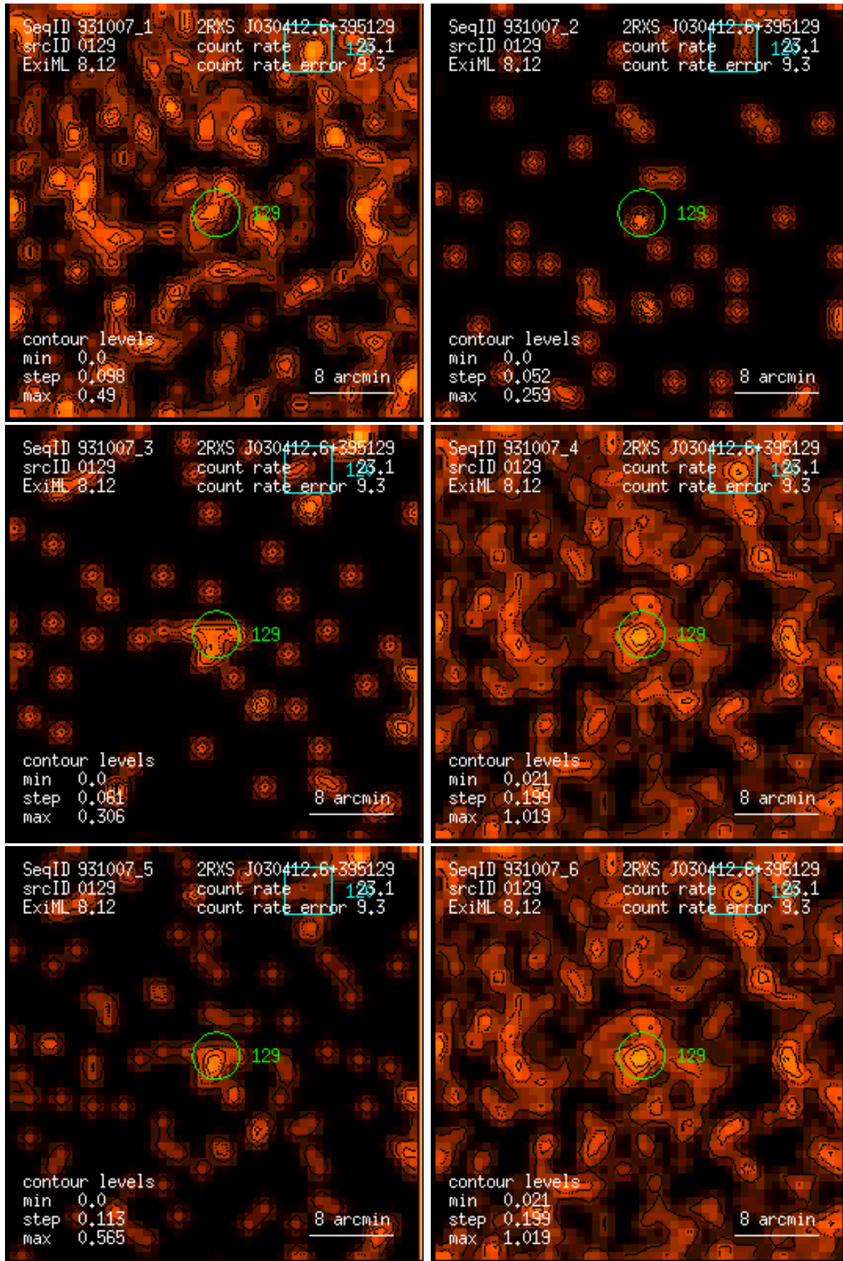
Figure 129: RASS 931007: detection 0129: band rate images, Gaussian filter: (1) PSPC channels 11 – 41, (2) 52 – 90, (3) 91 – 201, (4) 11 – 235, (5) 52 – 201, (6) 11 – 201. Broad band rates in counts/ks. Band rate contour levels in counts/ks/arcmin 2 .
