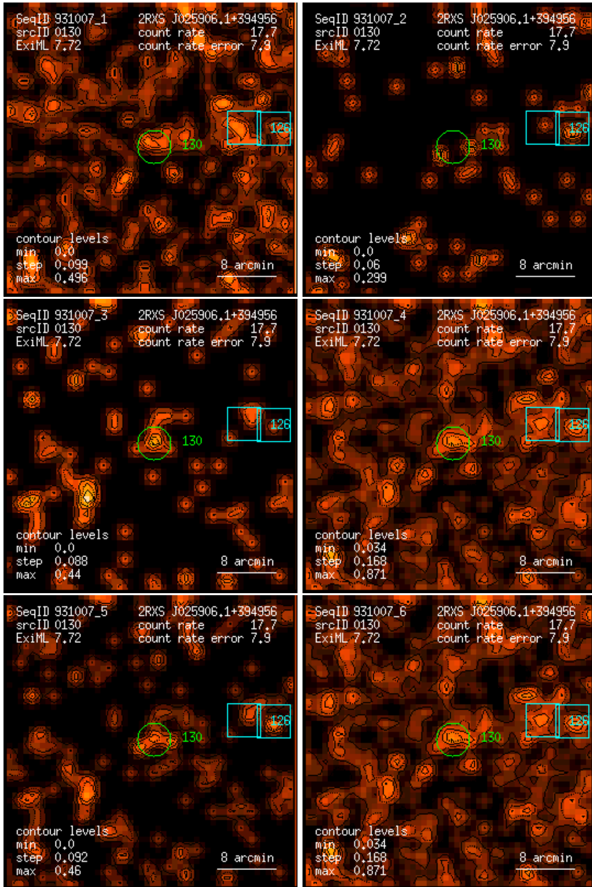
Figure 130: RASS 931007: detection 0130: band rate images, Gaussian filter: (1) PSPC channels 11 – 41, (2) 52 – 90, (3) 91 – 201, (4) 11 – 235, (5) 52 – 201, (6) 11 – 201. Broad band rates in counts/ks. Band rate contour levels in counts/ks/arcmin 2 .
