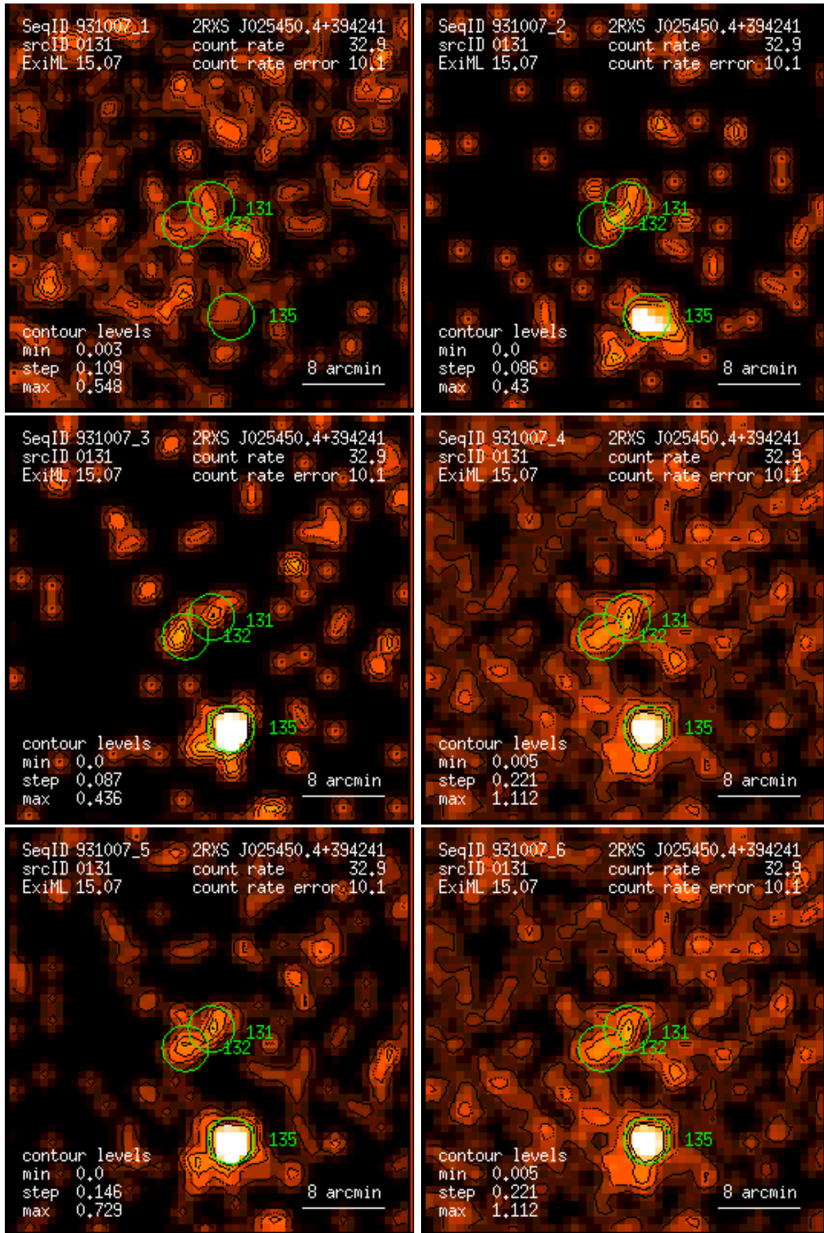
Figure 131: RASS 931007: detection 0131: band rate images, Gaussian filter: (1) PSPC channels 11 – 41, (2) 52 – 90, (3) 91 – 201, (4) 11 – 235, (5) 52 – 201, (6) 11 – 201. Broad band rates in counts/ks. Band rate contour levels in counts/ks/arcmin 2 .
