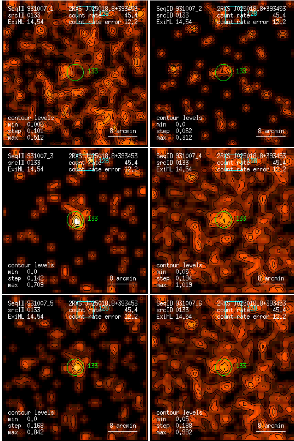
Figure 133: RASS 931007: detection 0133: band rate images, Gaussian filter: (1) PSPC channels 11 – 41, (2) 52 – 90, (3) 91 – 201, (4) 11 – 235, (5) 52 – 201, (6) 11 – 201. Broad band rates in counts/ks. Band rate contour levels in counts/ks/arcmin 2 .
