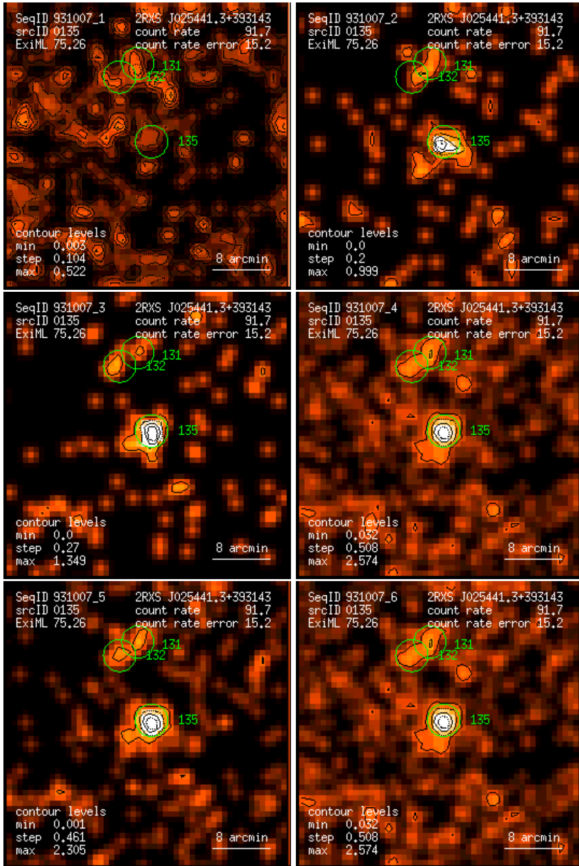
Figure 135: RASS 931007: detection 0135: band rate images, Gaussian filter: (1) PSPC channels 11 – 41, (2) 52 – 90, (3) 91 – 201, (4) 11 – 235, (5) 52 – 201, (6) 11 – 201. Broad band rates in counts/ks. Band rate contour levels in counts/ks/arcmin 2 .
