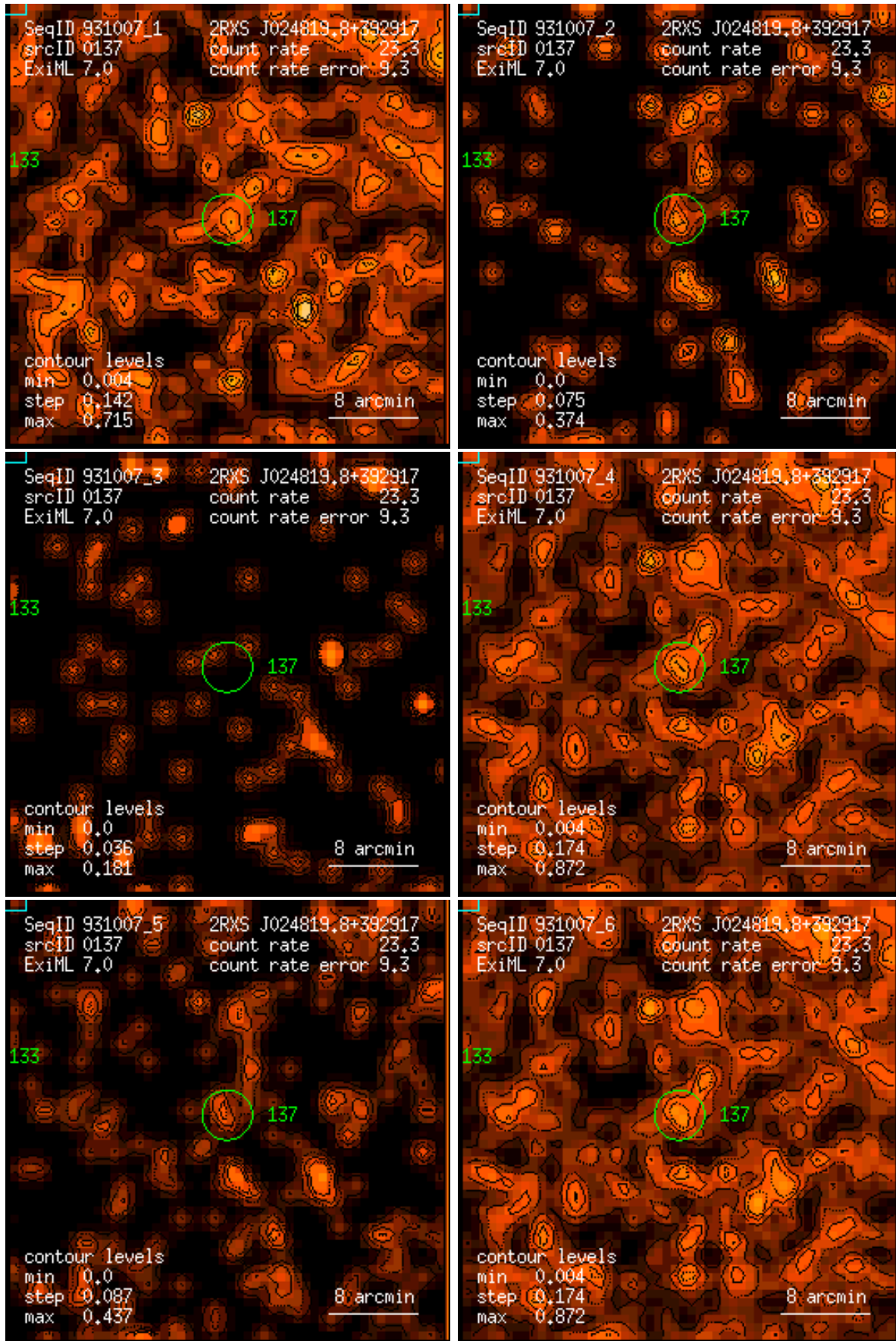
Figure 137: RASS 931007: detection 0137: band rate images, Gaussian filter: (1) PSPC channels 11 – 41, (2) 52 – 90, (3) 91 – 201, (4) 11 – 235, (5) 52 – 201, (6) 11 – 201. Broad band rates in counts/ks. Band rate contour levels in counts/ks/arcmin 2 .
