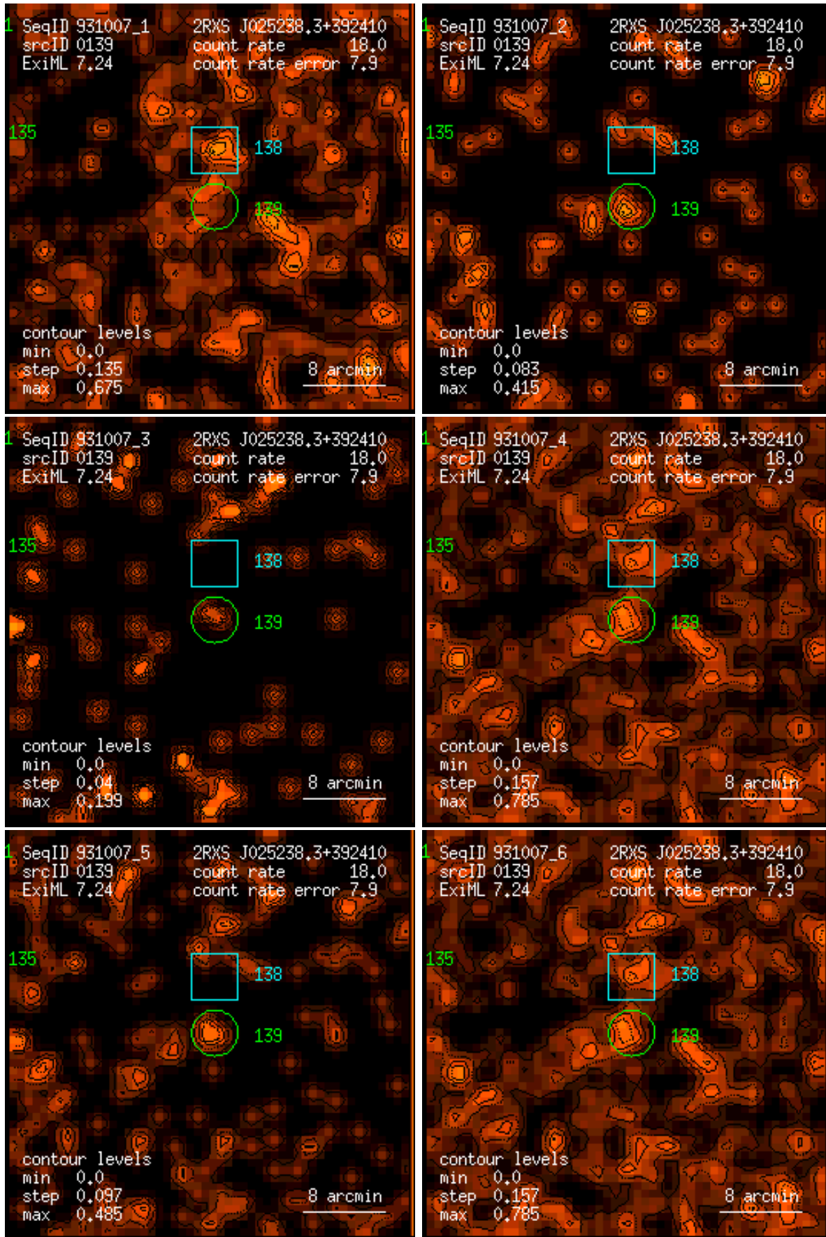
Figure 139: RASS 931007: detection 0139: band rate images, Gaussian filter: (1) PSPC channels 11 – 41, (2) 52 – 90, (3) 91 – 201, (4) 11 – 235, (5) 52 – 201, (6) 11 – 201. Broad band rates in counts/ks. Band rate contour levels in counts/ks/arcmin 2 .
