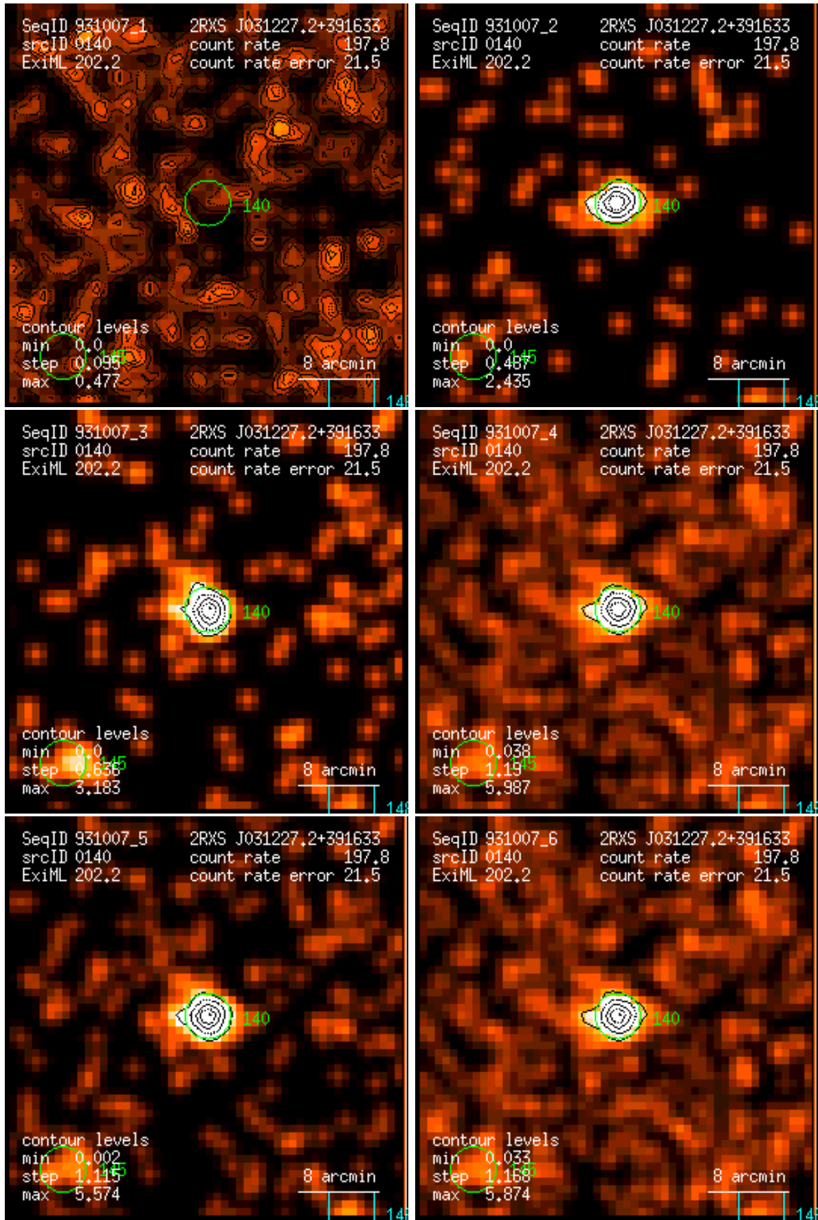
Figure 140: RASS 931007: detection 0140: band rate images, Gaussian filter: (1) PSPC channels 11 – 41, (2) 52 – 90, (3) 91 – 201, (4) 11 – 235, (5) 52 – 201, (6) 11 – 201. Broad band rates in counts/ks. Band rate contour levels in counts/ks/arcmin 2 .
