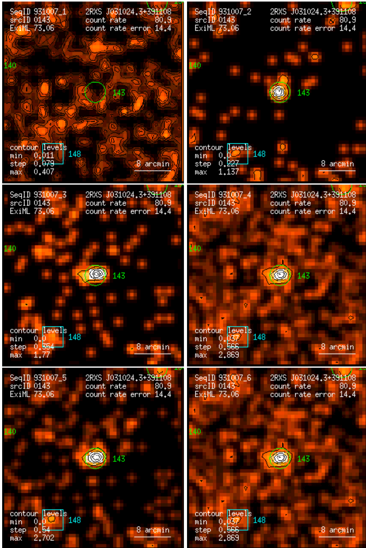
Figure 143: RASS 931007: detection 0143: band rate images, Gaussian filter: (1) PSPC channels 11 – 41, (2) 52 – 90, (3) 91 – 201, (4) 11 – 235, (5) 52 – 201, (6) 11 – 201. Broad band rates in counts/ks. Band rate contour levels in counts/ks/arcmin 2 .
