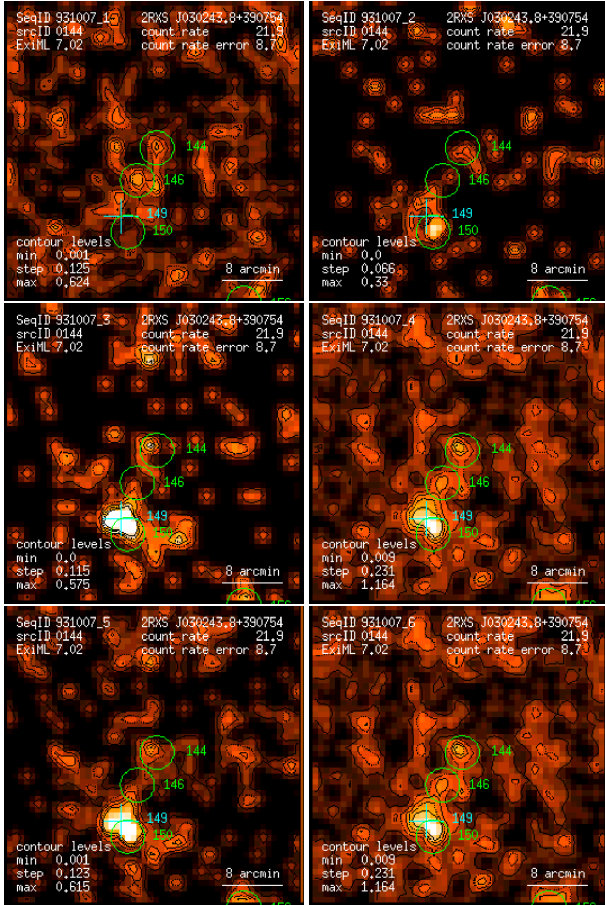
Figure 144: RASS 931007: detection 0144: band rate images, Gaussian filter: (1) PSPC channels 11 – 41, (2) 52 – 90, (3) 91 – 201, (4) 11 – 235, (5) 52 – 201, (6) 11 – 201. Broad band rates in counts/ks. Band rate contour levels in counts/ks/arcmin 2 .
