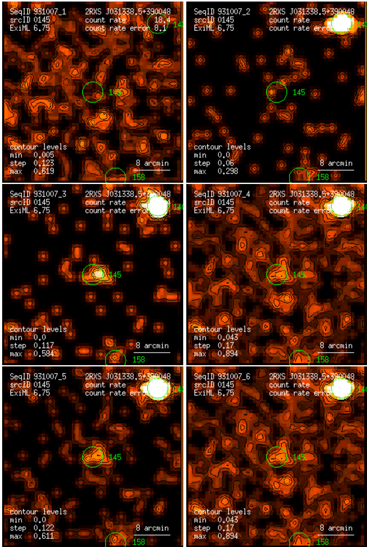
Figure 145: RASS 931007: detection 0145: band rate images, Gaussian filter: (1) PSPC channels 11 – 41, (2) 52 – 90, (3) 91 – 201, (4) 11 – 235, (5) 52 – 201, (6) 11 – 201. Broad band rates in counts/ks. Band rate contour levels in counts/ks/arcmin 2 .
