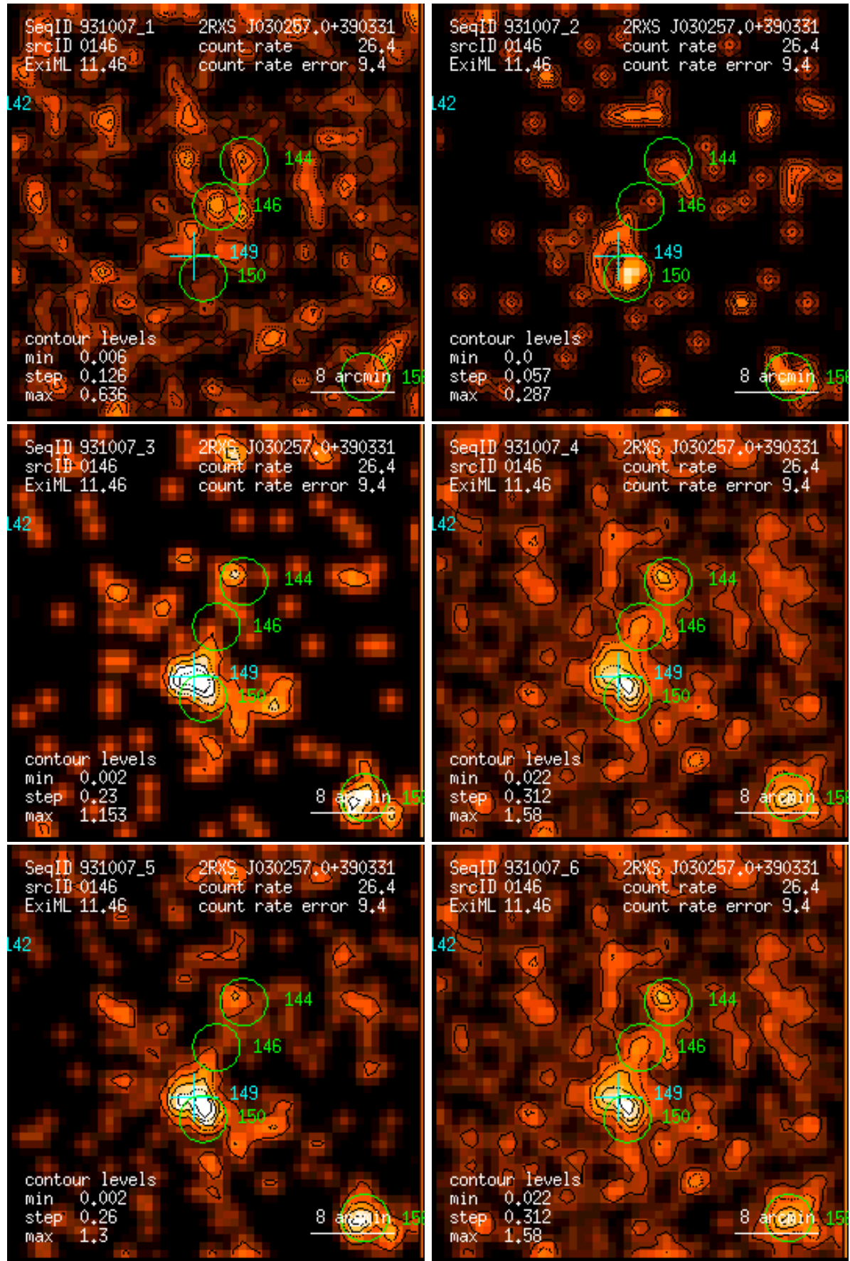
Figure 146: RASS 931007: detection 0146: band rate images, Gaussian filter: (1) PSPC channels 11 – 41, (2) 52 – 90, (3) 91 – 201, (4) 11 – 235, (5) 52 – 201, (6) 11 – 201. Broad band rates in counts/ks. Band rate contour levels in counts/ks/arcmin 2 .
