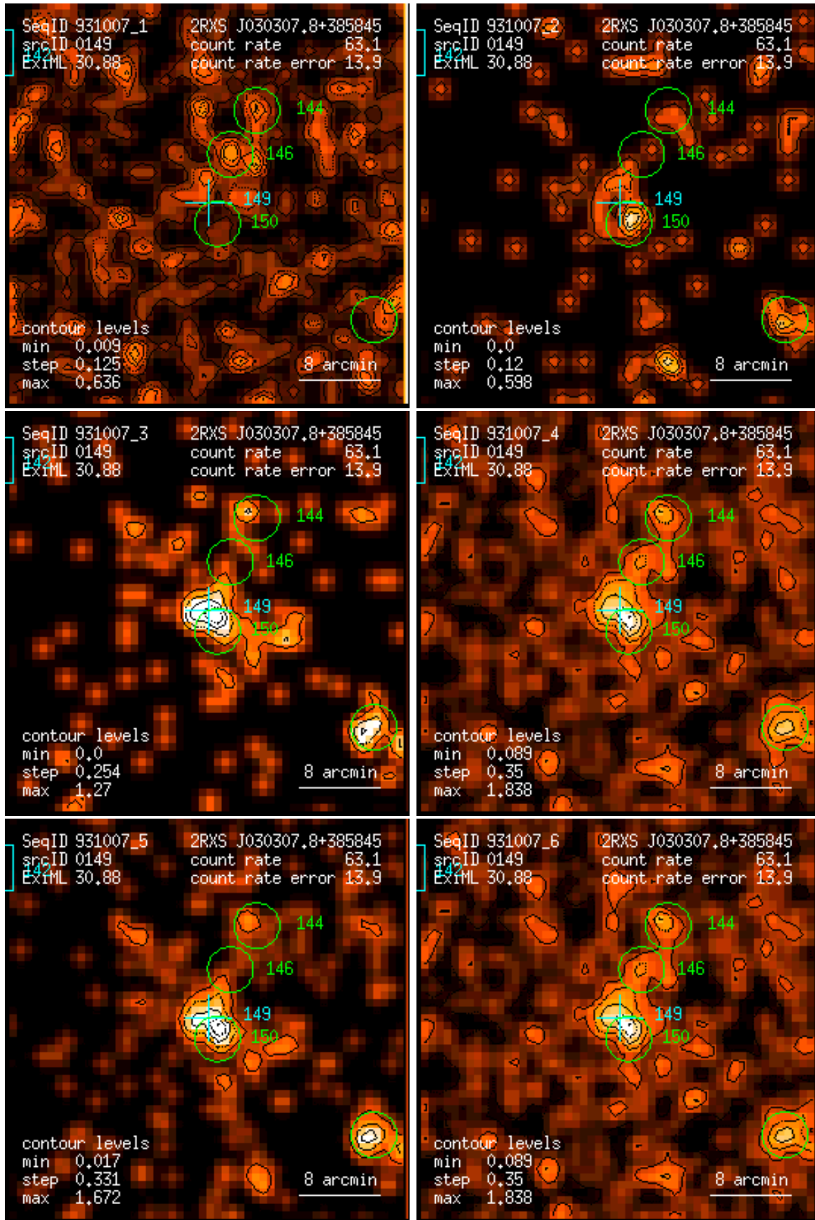
Figure 149: RASS 931007: detection 0149: band rate images, Gaussian filter: (1) PSPC channels 11 – 41, (2) 52 – 90, (3) 91 – 201, (4) 11 – 235, (5) 52 – 201, (6) 11 – 201. Broad band rates in counts/ks. Band rate contour levels in counts/ks/arcmin 2 .
