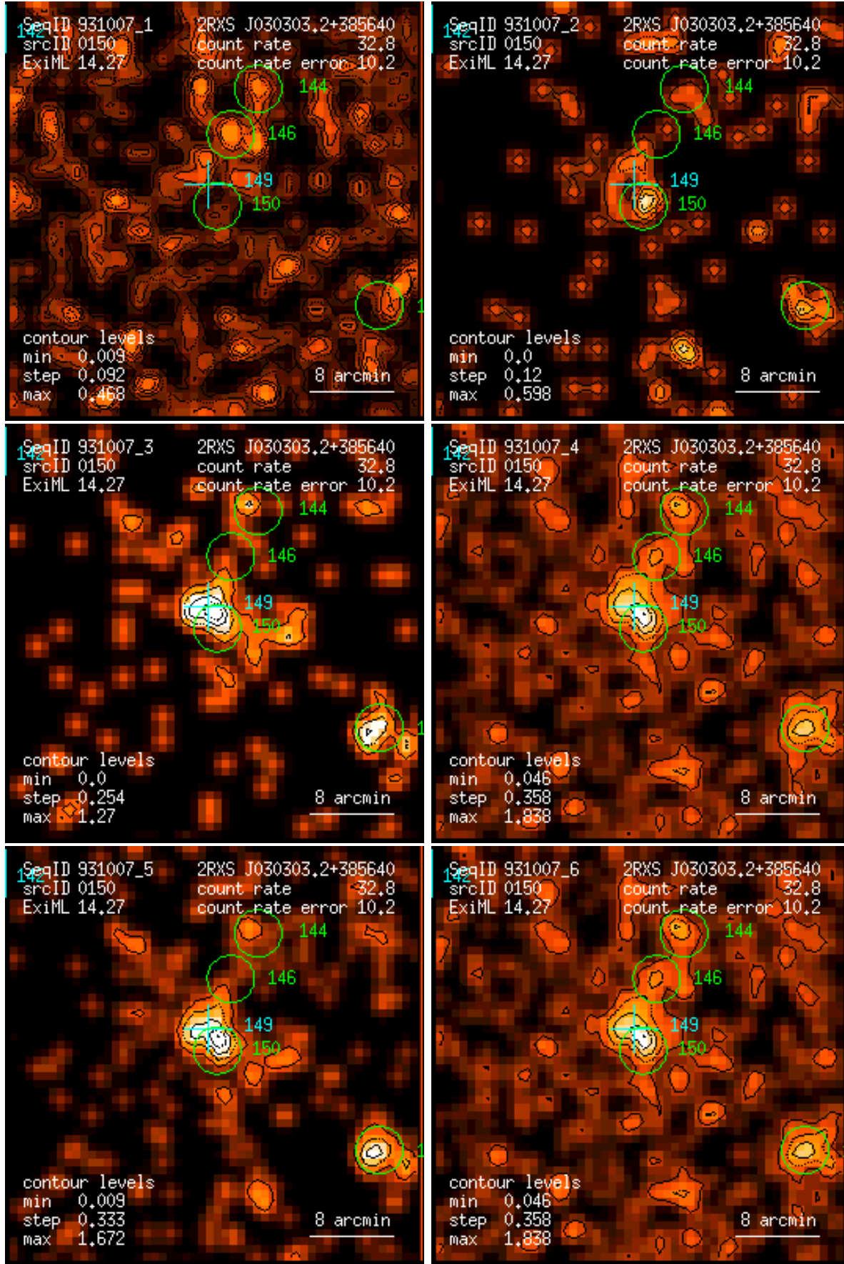
Figure 150: RASS 931007: detection 0150: band rate images, Gaussian filter: (1) PSPC channels 11 – 41, (2) 52 – 90, (3) 91 – 201, (4) 11 – 235, (5) 52 – 201, (6) 11 – 201. Broad band rates in counts/ks. Band rate contour levels in counts/ks/arcmin 2 .
