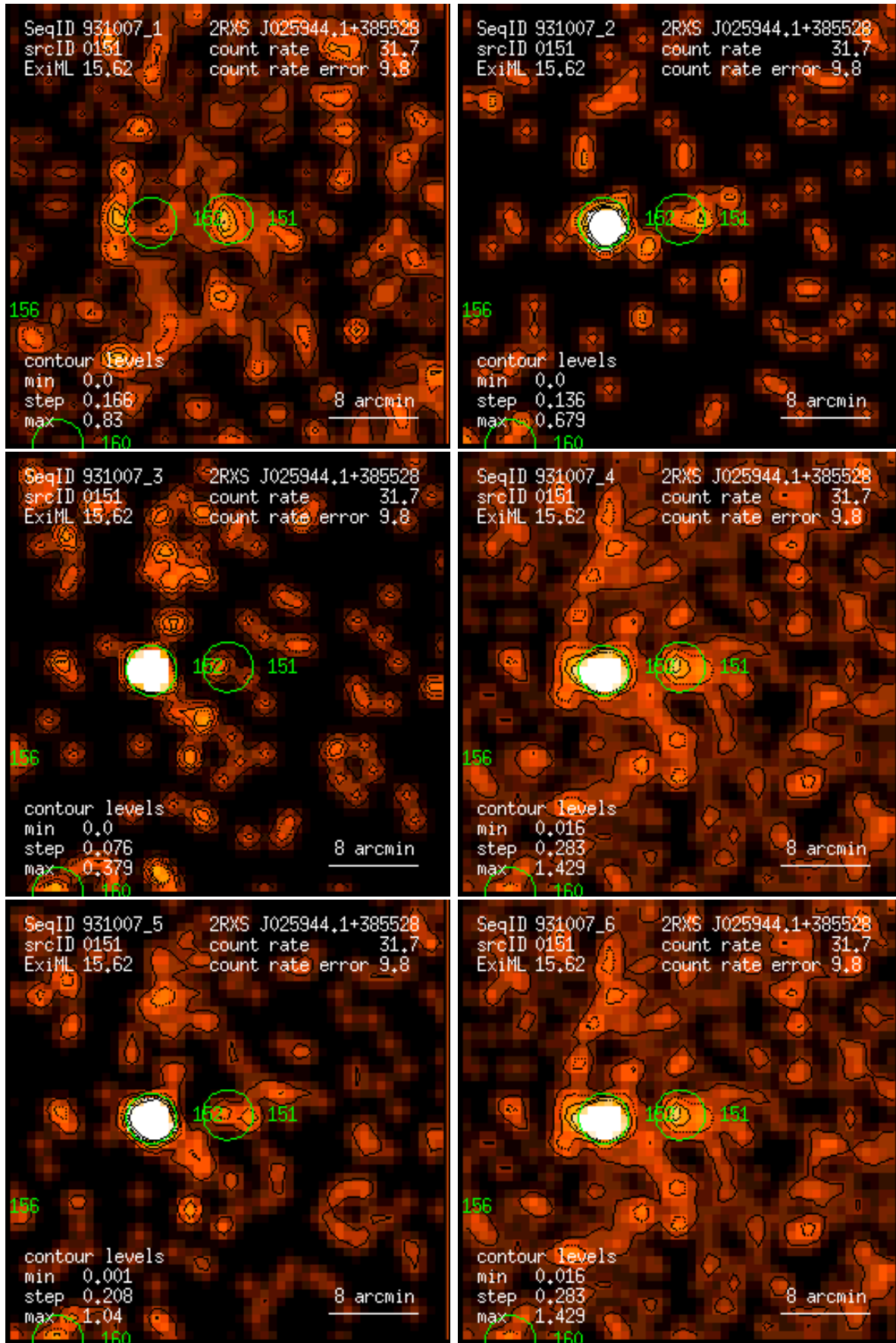
Figure 151: RASS 931007: detection 0151: band rate images, Gaussian filter: (1) PSPC channels 11 – 41, (2) 52 – 90, (3) 91 – 201, (4) 11 – 235, (5) 52 – 201, (6) 11 – 201. Broad band rates in counts/ks. Band rate contour levels in counts/ks/arcmin 2 .
