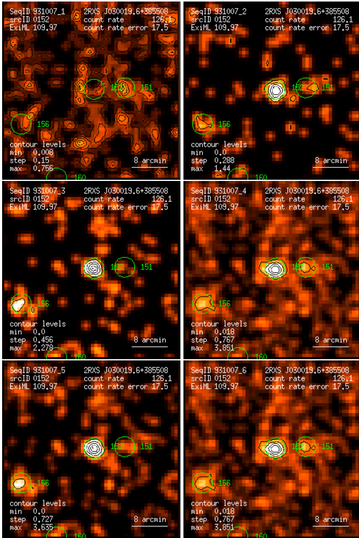
Figure 152: RASS 931007: detection 0152: band rate images, Gaussian filter: (1) PSPC channels 11 – 41, (2) 52 – 90, (3) 91 – 201, (4) 11 – 235, (5) 52 – 201, (6) 11 – 201. Broad band rates in counts/ks. Band rate contour levels in counts/ks/arcmin 2 .
