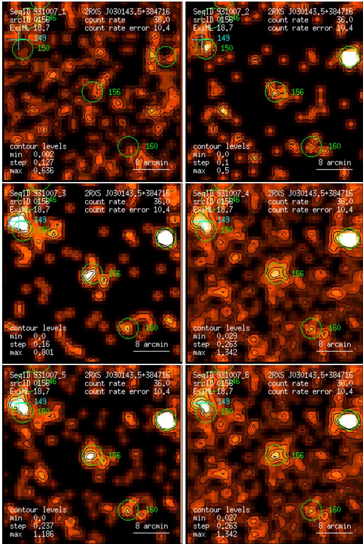
Figure 156: RASS 931007: detection 0156: band rate images, Gaussian filter: (1) PSPC channels 11 – 41, (2) 52 – 90, (3) 91 – 201, (4) 11 – 235, (5) 52 – 201, (6) 11 – 201. Broad band rates in counts/ks. Band rate contour levels in counts/ks/arcmin 2 .
