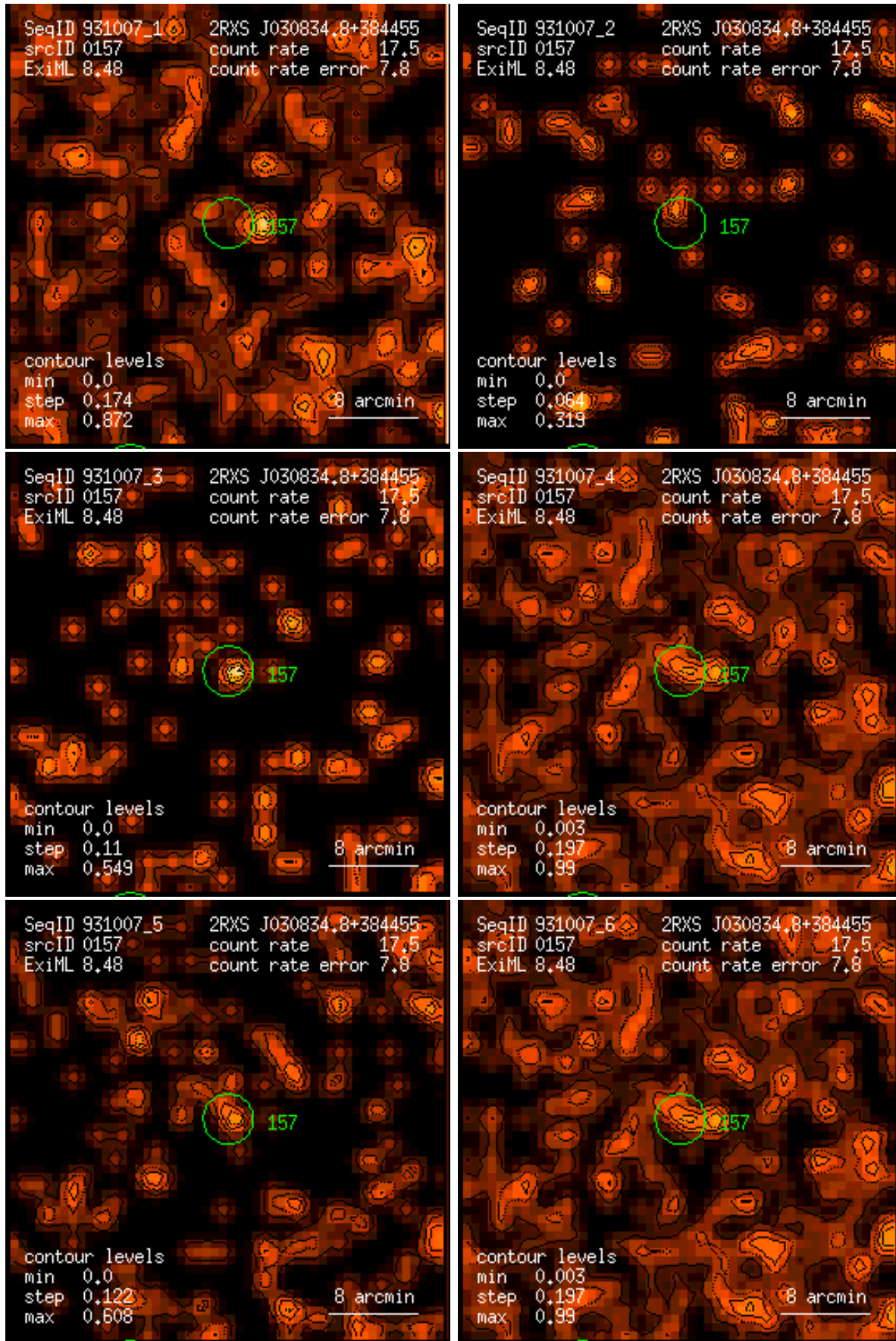
Figure 157: RASS 931007: detection 0157: band rate images, Gaussian filter: (1) PSPC channels 11 – 41, (2) 52 – 90, (3) 91 – 201, (4) 11 – 235, (5) 52 – 201, (6) 11 – 201. Broad band rates in counts/ks. Band rate contour levels in counts/ks/arcmin 2 .
