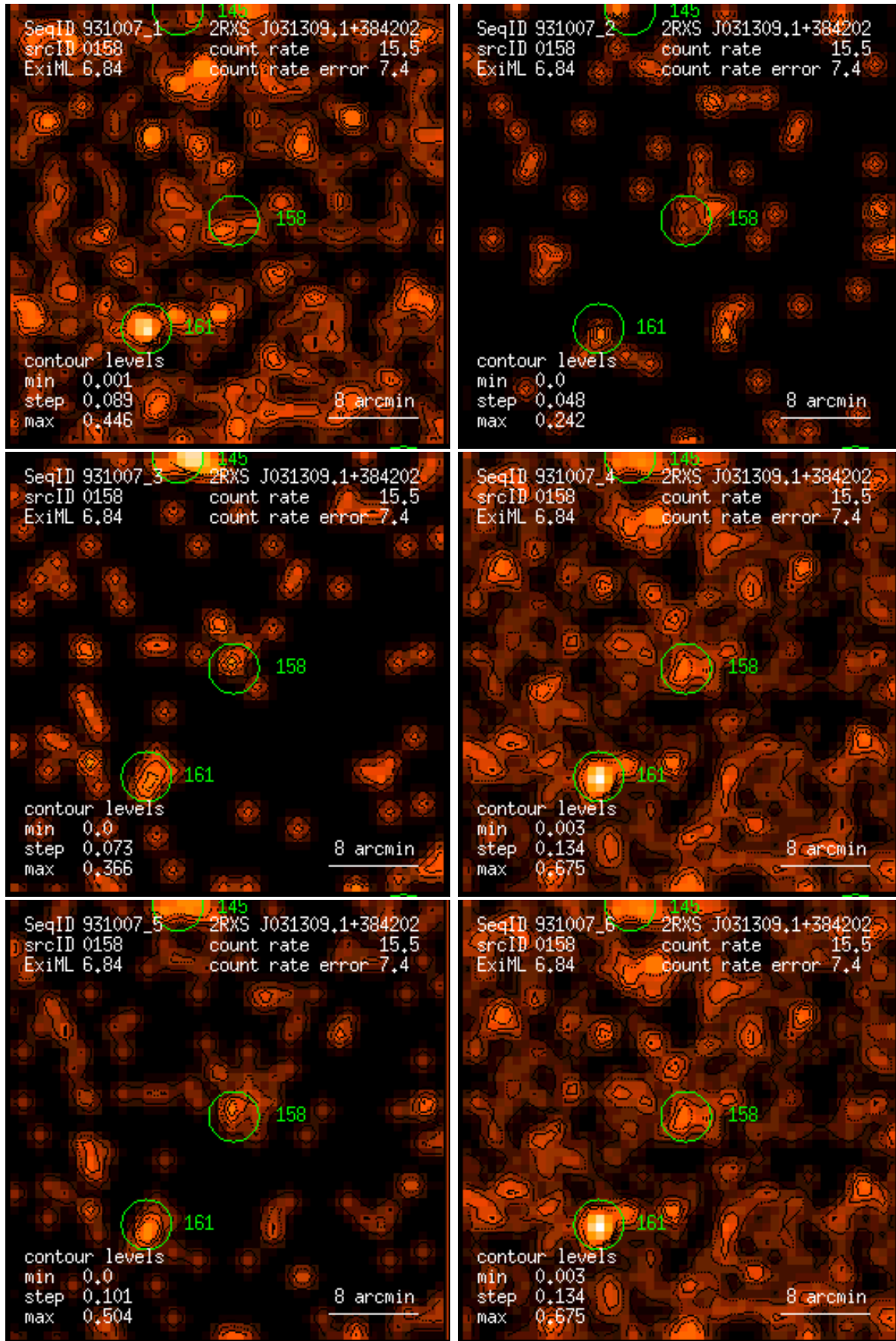
Figure 158: RASS 931007: detection 0158: band rate images, Gaussian filter: (1) PSPC channels 11 – 41, (2) 52 – 90, (3) 91 – 201, (4) 11 – 235, (5) 52 – 201, (6) 11 – 201. Broad band rates in counts/ks. Band rate contour levels in counts/ks/arcmin 2 .
