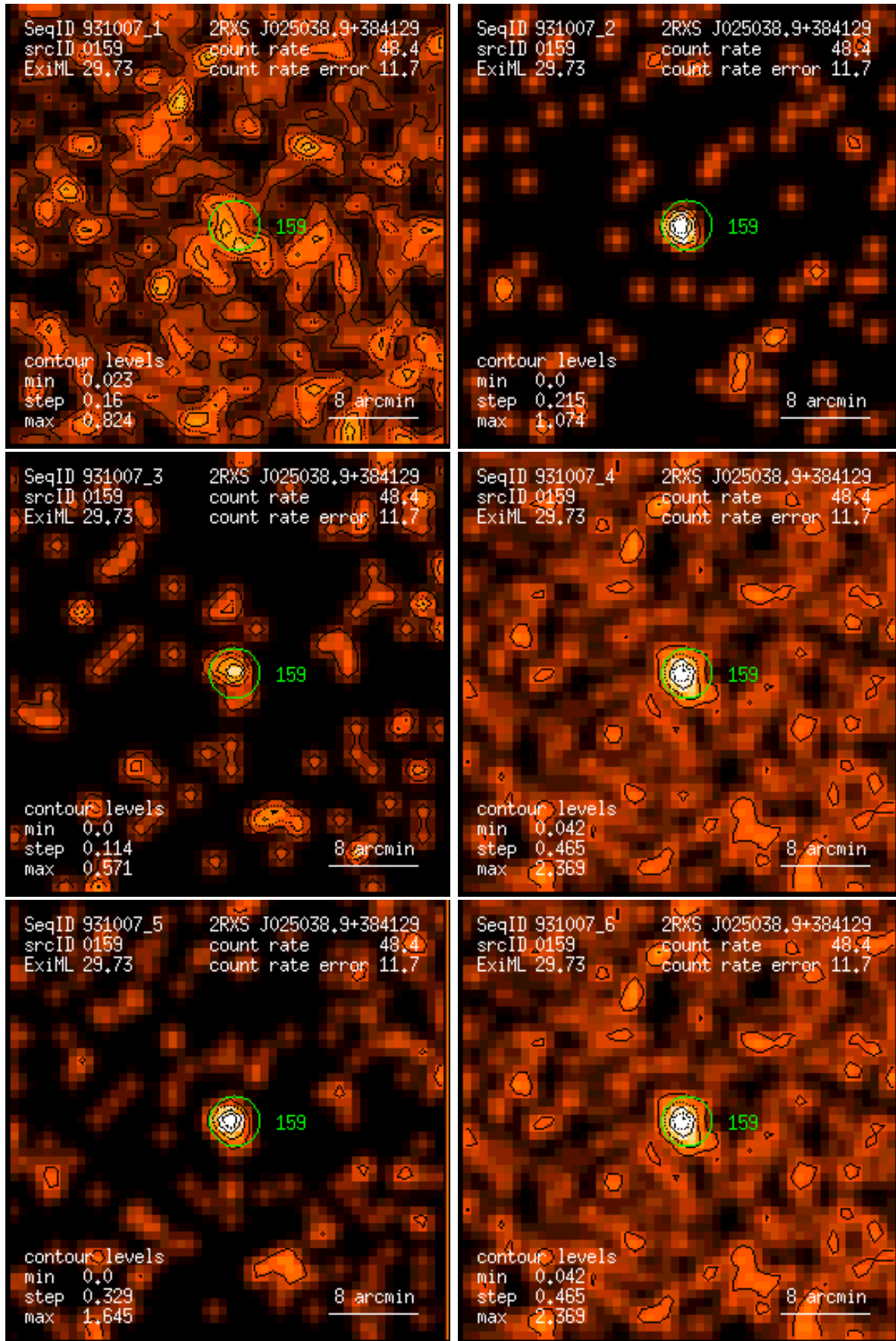
Figure 159: RASS 931007: detection 0159: band rate images, Gaussian filter: (1) PSPC channels 11 – 41, (2) 52 – 90, (3) 91 – 201, (4) 11 – 235, (5) 52 – 201, (6) 11 – 201. Broad band rates in counts/ks. Band rate contour levels in counts/ks/arcmin 2 .
