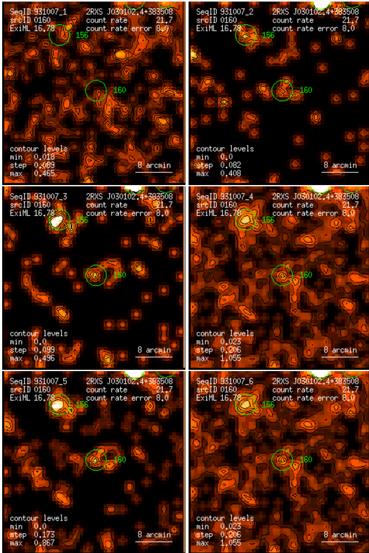
Figure 160: RASS 931007: detection 0160: band rate images, Gaussian filter: (1) PSPC channels 11 – 41, (2) 52 – 90, (3) 91 – 201, (4) 11 – 235, (5) 52 – 201, (6) 11 – 201. Broad band rates in counts/ks. Band rate contour levels in counts/ks/arcmin 2 .
