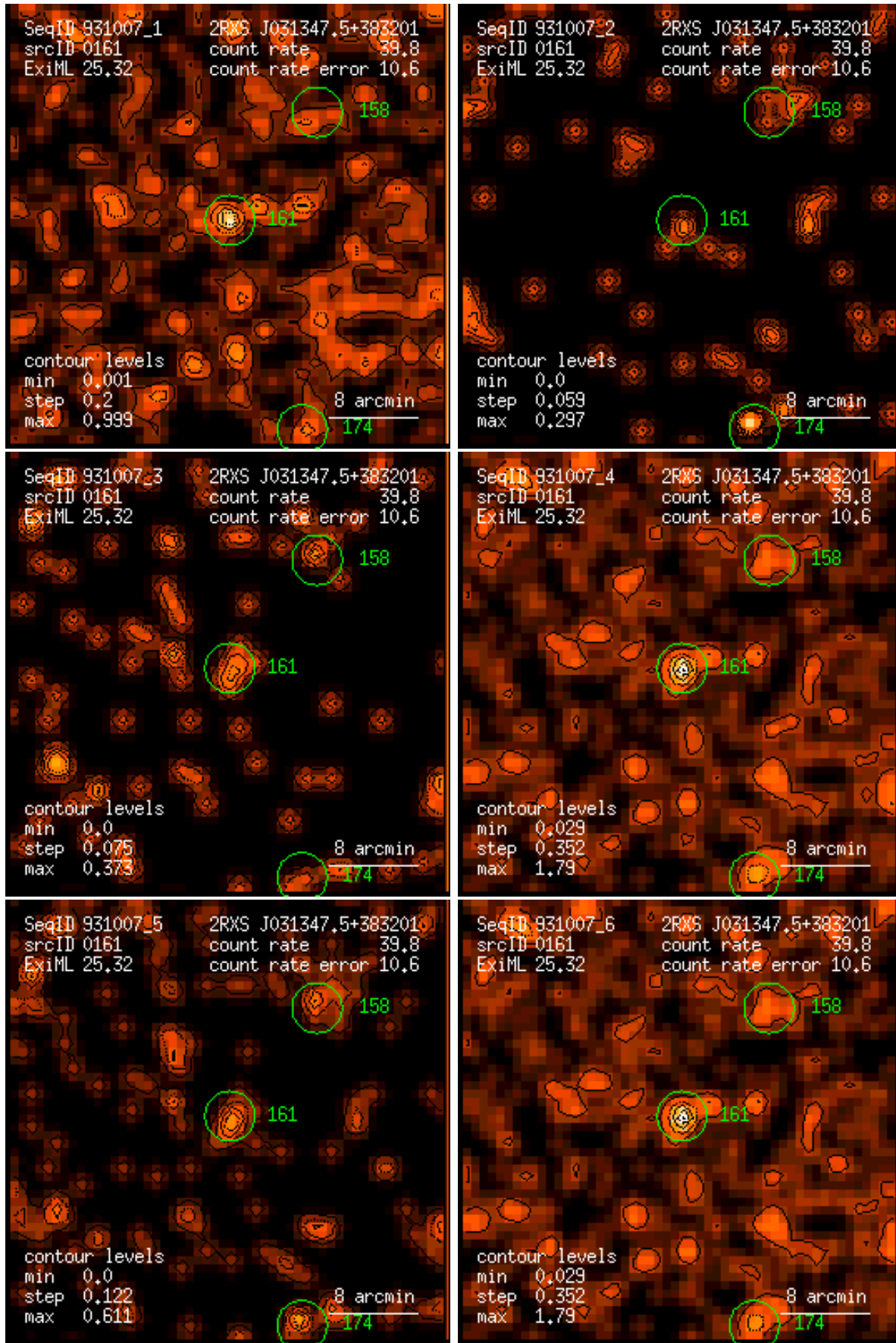
Figure 161: RASS 931007: detection 0161: band rate images, Gaussian filter: (1) PSPC channels 11 – 41, (2) 52 – 90, (3) 91 – 201, (4) 11 – 235, (5) 52 – 201, (6) 11 – 201. Broad band rates in counts/ks. Band rate contour levels in counts/ks/arcmin 2 .
