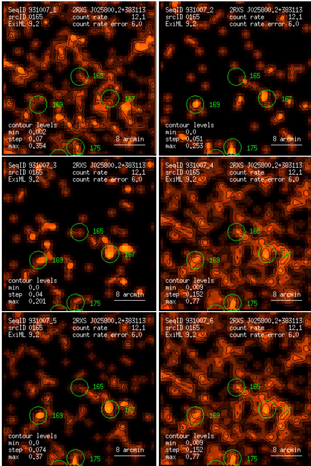
Figure 165: RASS 931007: detection 0165: band rate images, Gaussian filter: (1) PSPC channels 11 – 41, (2) 52 – 90, (3) 91 – 201, (4) 11 – 235, (5) 52 – 201, (6) 11 – 201. Broad band rates in counts/ks. Band rate contour levels in counts/ks/arcmin 2 .
