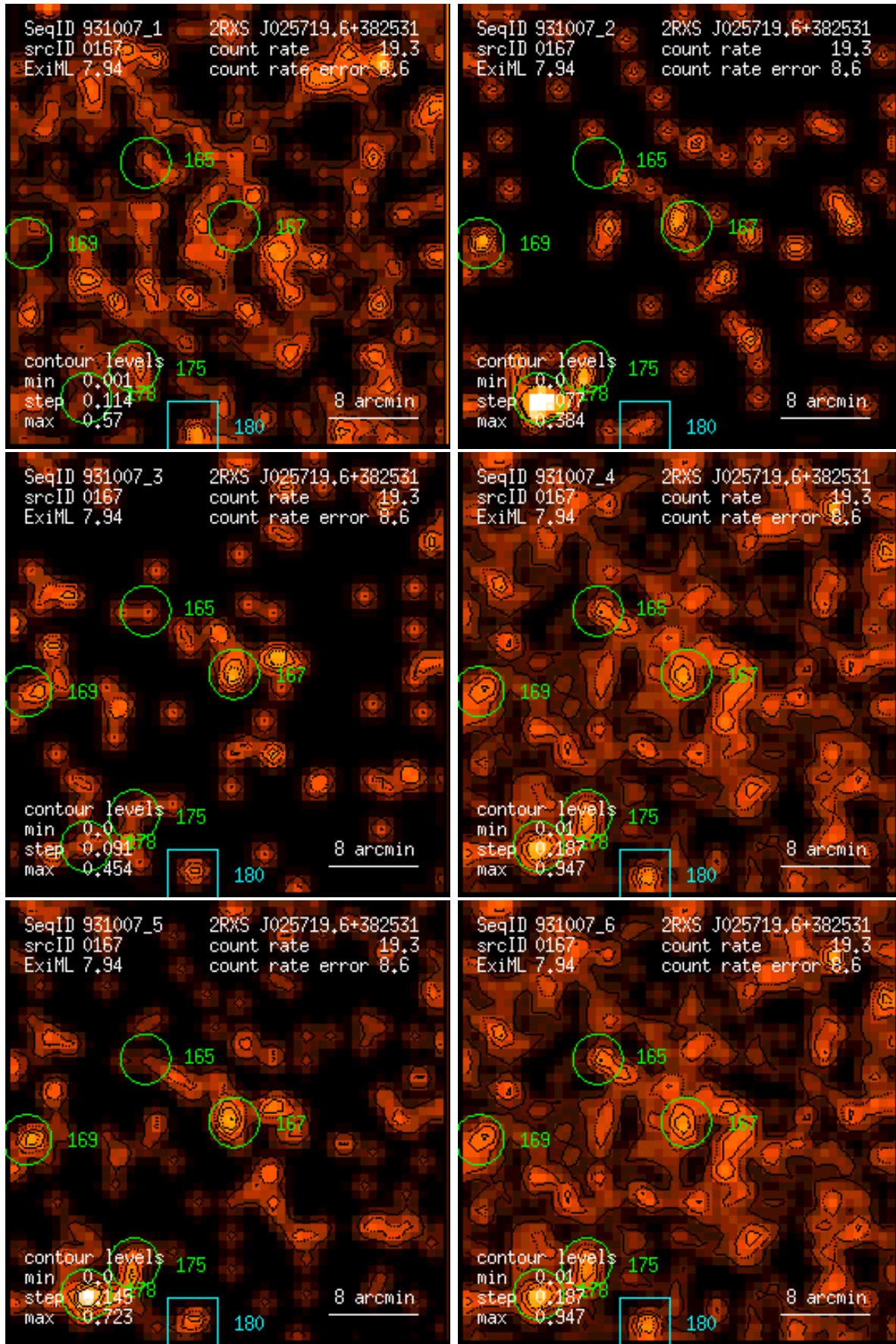
Figure 167: RASS 931007: detection 0167: band rate images, Gaussian filter: (1) PSPC channels 11 – 41, (2) 52 – 90, (3) 91 – 201, (4) 11 – 235, (5) 52 – 201, (6) 11 – 201. Broad band rates in counts/ks. Band rate contour levels in counts/ks/arcmin 2 .
