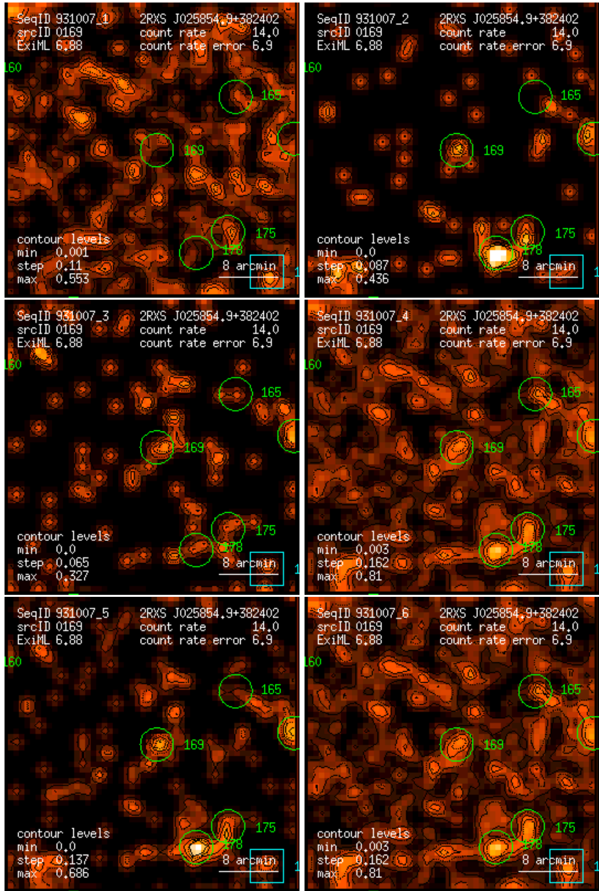
Figure 169: RASS 931007: detection 0169: band rate images, Gaussian filter: (1) PSPC channels 11 – 41, (2) 52 – 90, (3) 91 – 201, (4) 11 – 235, (5) 52 – 201, (6) 11 – 201. Broad band rates in counts/ks. Band rate contour levels in counts/ks/arcmin 2 .
