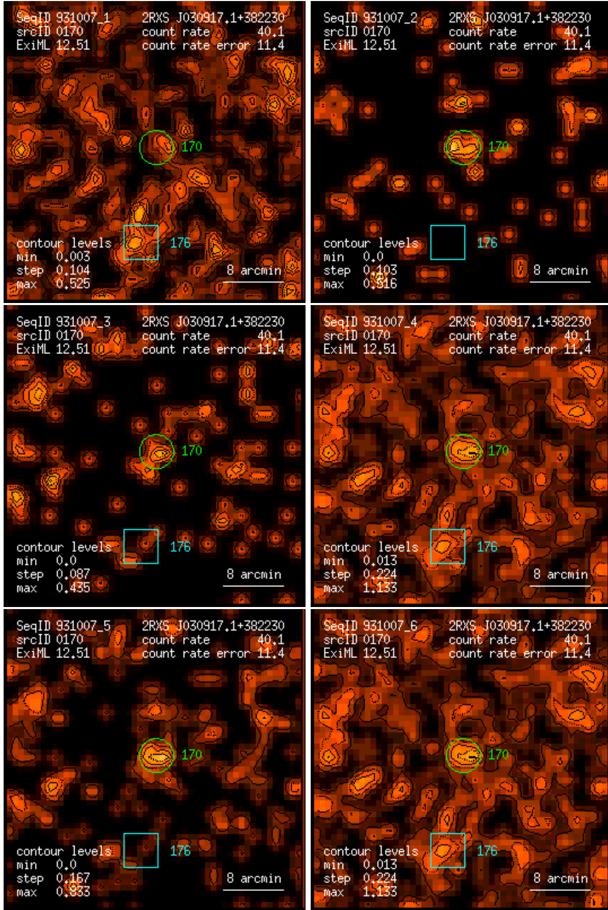
Figure 170: RASS 931007: detection 0170: band rate images, Gaussian filter: (1) PSPC channels 11 – 41, (2) 52 – 90, (3) 91 – 201, (4) 11 – 235, (5) 52 – 201, (6) 11 – 201. Broad band rates in counts/ks. Band rate contour levels in counts/ks/arcmin 2 .
