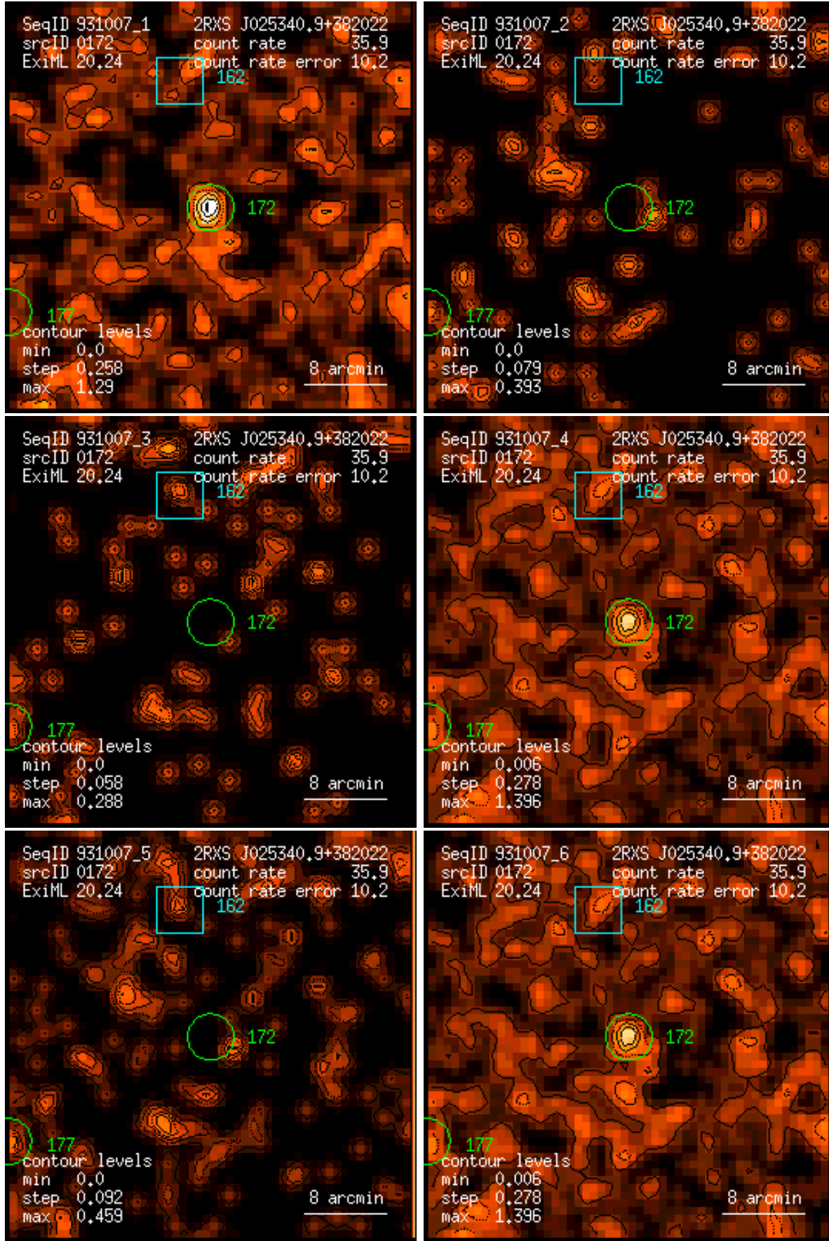
Figure 172: RASS 931007: detection 0172: band rate images, Gaussian filter: (1) PSPC channels 11 – 41, (2) 52 – 90, (3) 91 – 201, (4) 11 – 235, (5) 52 – 201, (6) 11 – 201. Broad band rates in counts/ks. Band rate contour levels in counts/ks/arcmin 2 .
