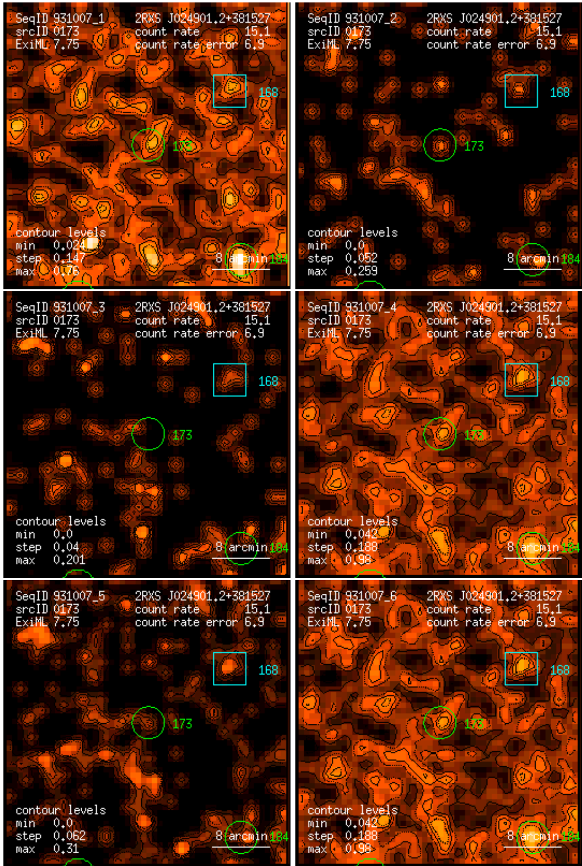
Figure 173: RASS 931007: detection 0173: band rate images, Gaussian filter: (1) PSPC channels 11 – 41, (2) 52 – 90, (3) 91 – 201, (4) 11 – 235, (5) 52 – 201, (6) 11 – 201. Broad band rates in counts/ks. Band rate contour levels in counts/ks/arcmin 2 .
