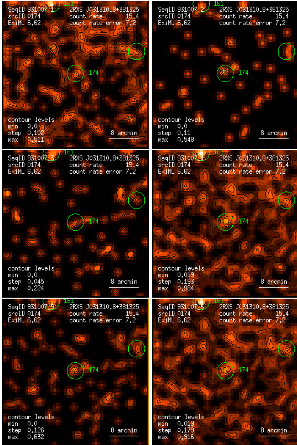
Figure 174: RASS 931007: detection 0174: band rate images, Gaussian filter: (1) PSPC channels 11 – 41, (2) 52 – 90, (3) 91 – 201, (4) 11 – 235, (5) 52 – 201, (6) 11 – 201. Broad band rates in counts/ks. Band rate contour levels in counts/ks/arcmin 2 .
