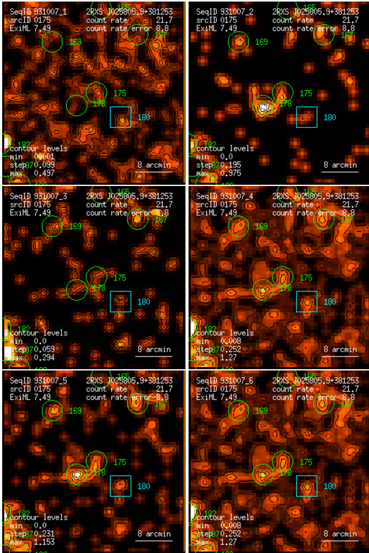
Figure 175: RASS 931007: detection 0175: band rate images, Gaussian filter: (1) PSPC channels 11 – 41, (2) 52 – 90, (3) 91 – 201, (4) 11 – 235, (5) 52 – 201, (6) 11 – 201. Broad band rates in counts/ks. Band rate contour levels in counts/ks/arcmin 2 .
