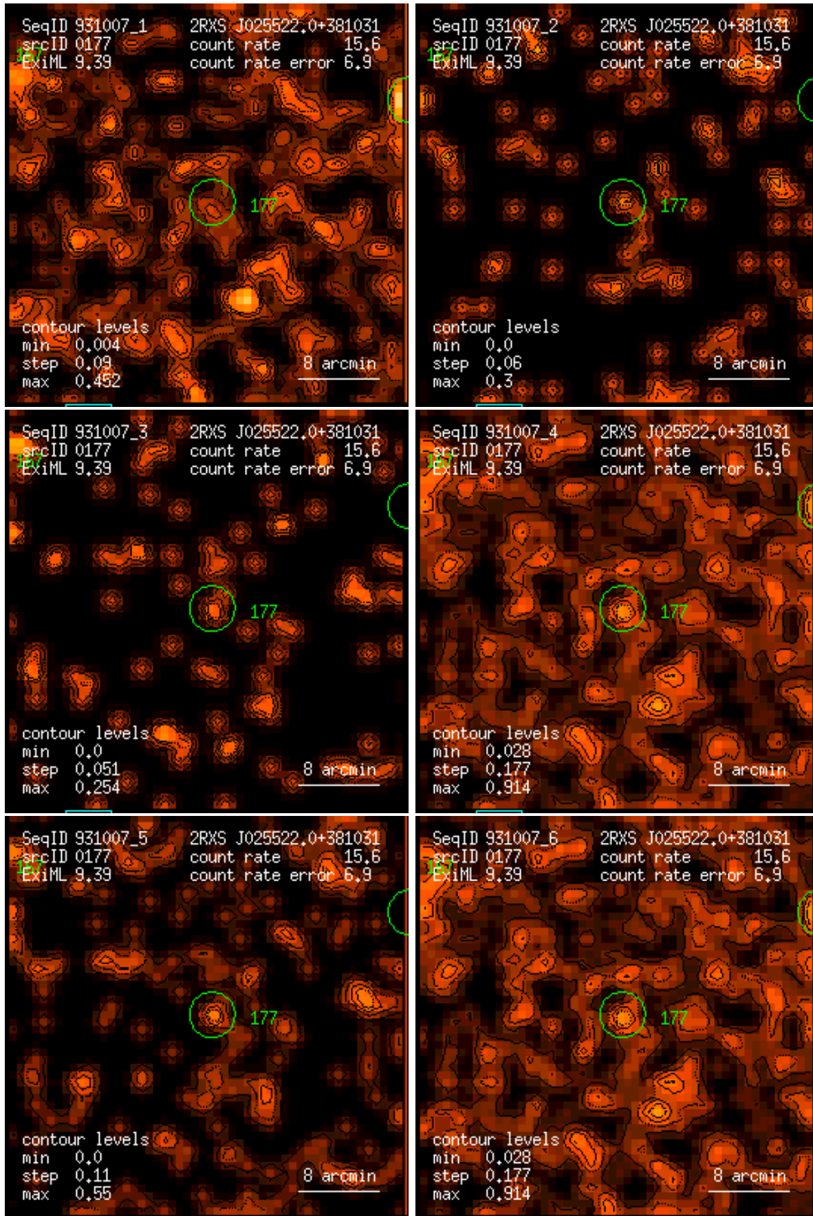
Figure 177: RASS 931007: detection 0177: band rate images, Gaussian filter: (1) PSPC channels 11 – 41, (2) 52 – 90, (3) 91 – 201, (4) 11 – 235, (5) 52 – 201, (6) 11 – 201. Broad band rates in counts/ks. Band rate contour levels in counts/ks/arcmin 2 .
