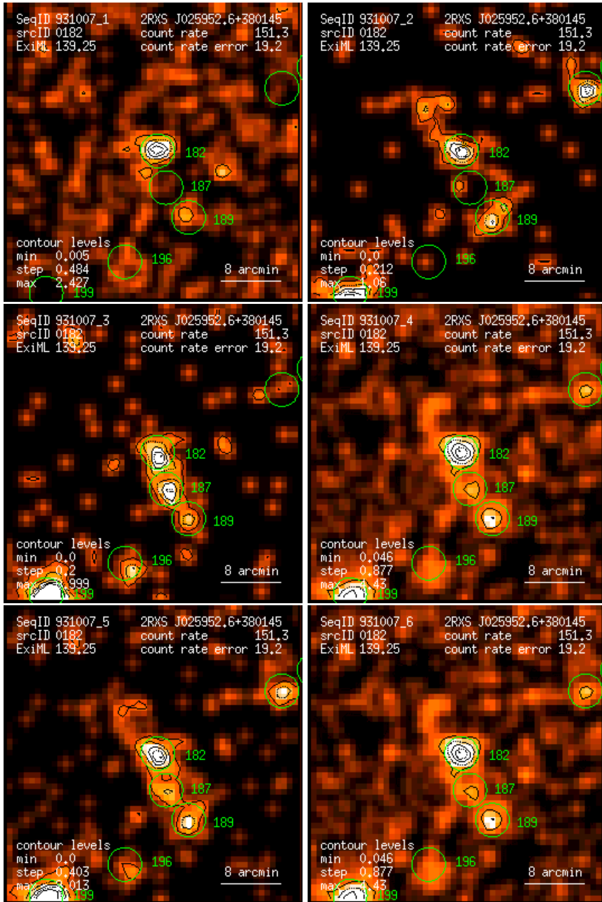
Figure 182: RASS 931007: detection 0182: band rate images, Gaussian filter: (1) PSPC channels 11 – 41, (2) 52 – 90, (3) 91 – 201, (4) 11 – 235, (5) 52 – 201, (6) 11 – 201. Broad band rates in counts/ks. Band rate contour levels in counts/ks/arcmin 2 .
