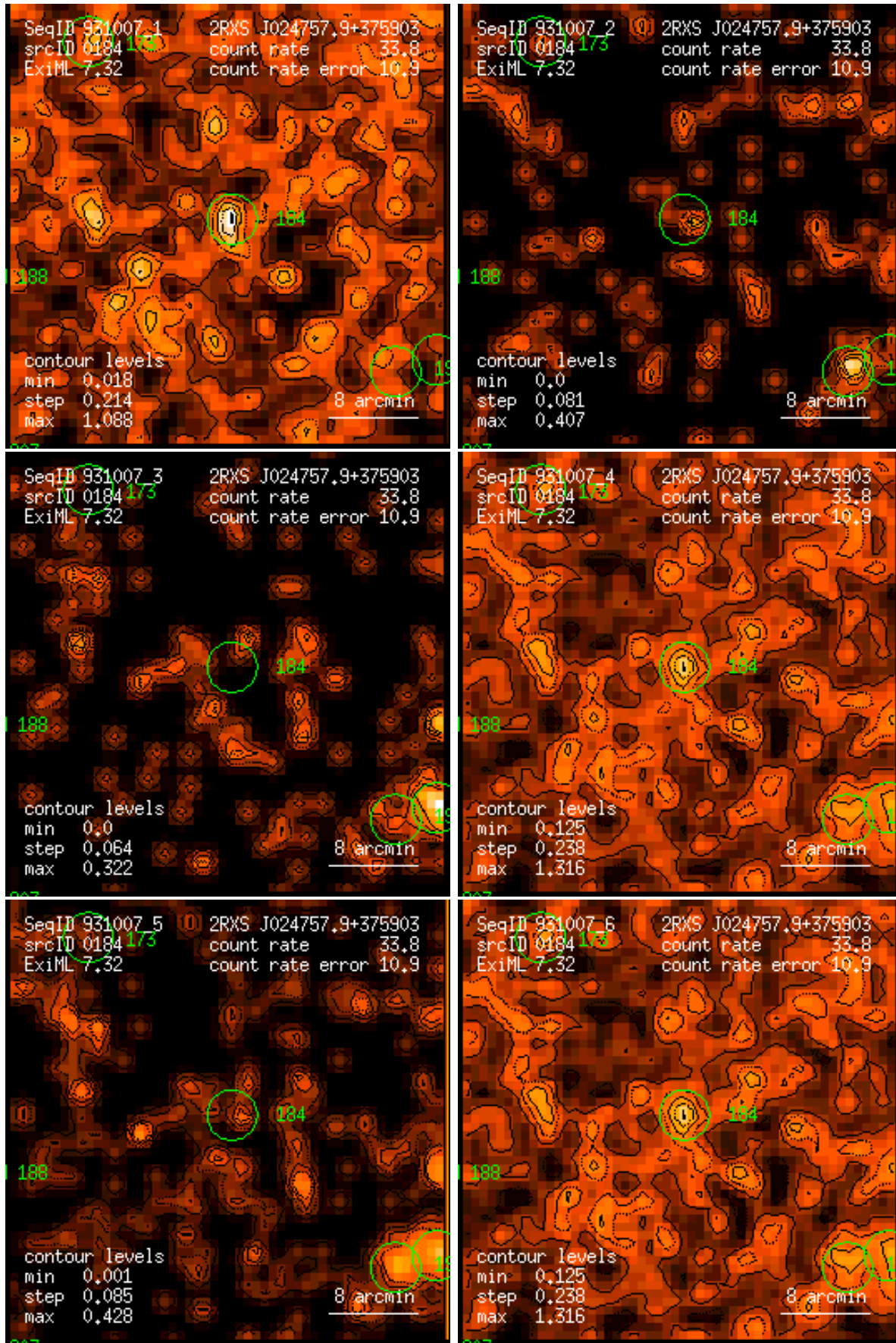
Figure 184: RASS 931007: detection 0184: band rate images, Gaussian filter: (1) PSPC channels 11 – 41, (2) 52 – 90, (3) 91 – 201, (4) 11 – 235, (5) 52 – 201, (6) 11 – 201. Broad band rates in counts/ks. Band rate contour levels in counts/ks/arcmin 2 .
