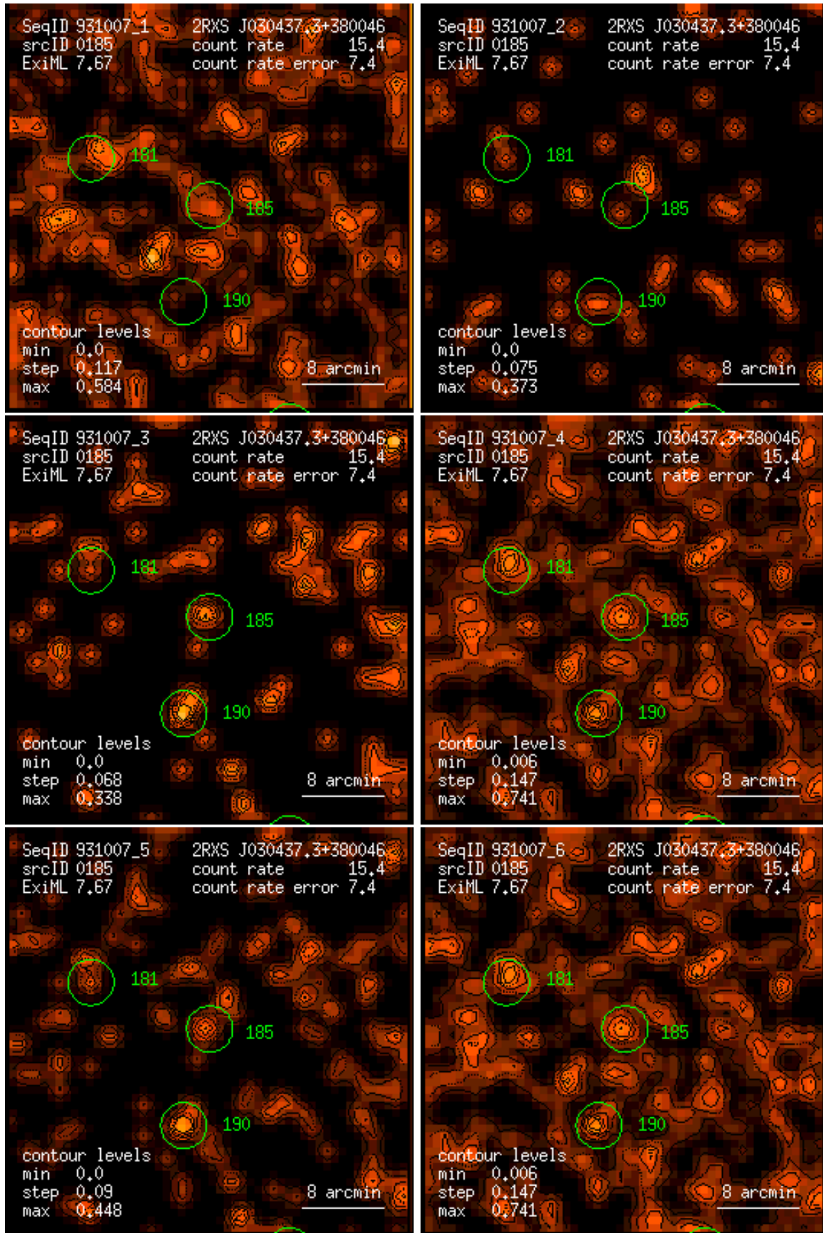
Figure 185: RASS 931007: detection 0185: band rate images, Gaussian filter: (1) PSPC channels 11 – 41, (2) 52 – 90, (3) 91 – 201, (4) 11 – 235, (5) 52 – 201, (6) 11 – 201. Broad band rates in counts/ks. Band rate contour levels in counts/ks/arcmin 2 .
