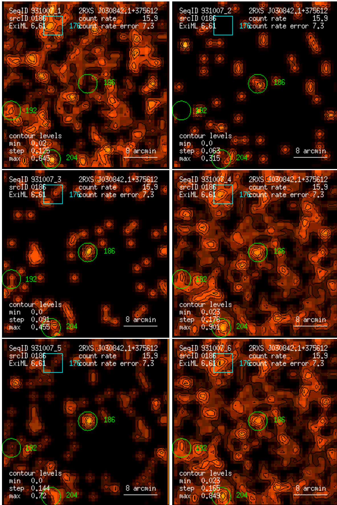
Figure 186: RASS 931007: detection 0186: band rate images, Gaussian filter: (1) PSPC channels 11 – 41, (2) 52 – 90, (3) 91 – 201, (4) 11 – 235, (5) 52 – 201, (6) 11 – 201. Broad band rates in counts/ks. Band rate contour levels in counts/ks/arcmin 2 .
