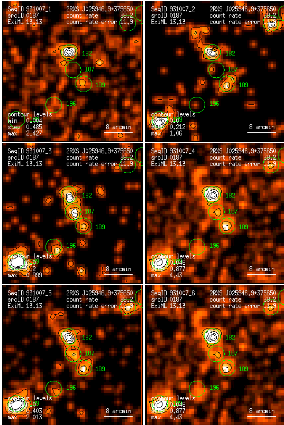
Figure 187: RASS 931007: detection 0187: band rate images, Gaussian filter: (1) PSPC channels 11 – 41, (2) 52 – 90, (3) 91 – 201, (4) 11 – 235, (5) 52 – 201, (6) 11 – 201. Broad band rates in counts/ks. Band rate contour levels in counts/ks/arcmin 2 .
